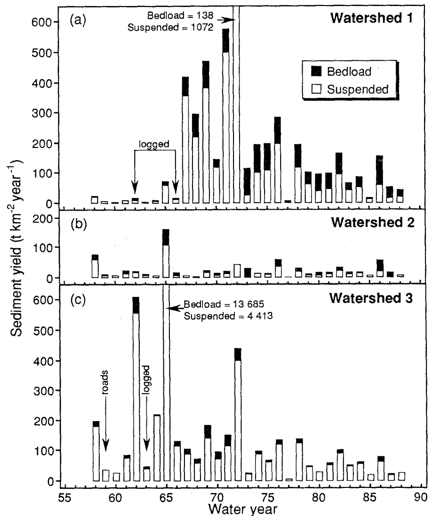
FIG. 1 Annual sediment yields for Watersheds 1, 2, and 3 for WY 1958-1988.
