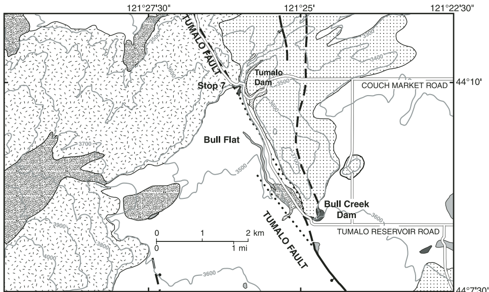
Figure 26. Geology of the Bull Flat–Tumalo Dam area. Illustration from Sherrod et al. (2002).
