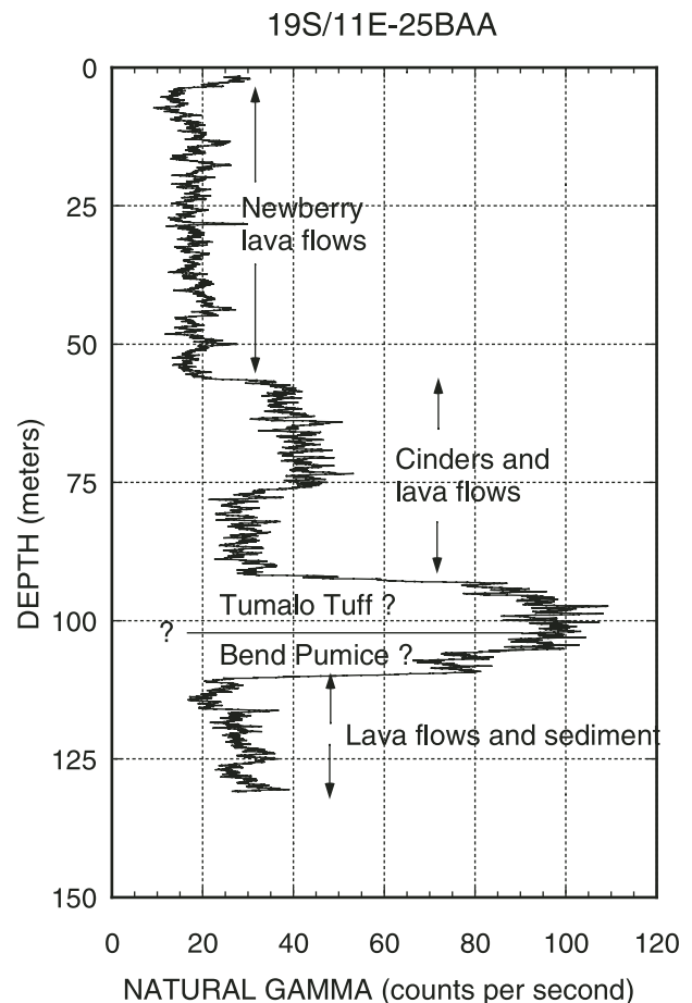
Figure 33. Natural gamma log and inferred stratigraphy in a well east of U.S. Highway 97 near Lava Butte. From Sherrod et al. (2002).
