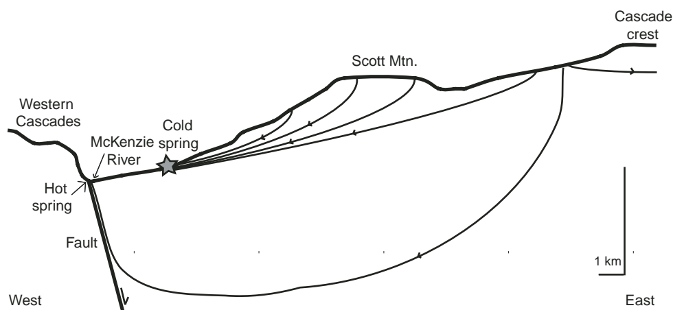
Figure 15. Cross section showing conceptual groundwater flow paths from the Cascade crest to the Western Cascades. Hot springs occur where deep groundwater flow paths are interrupted by faults (Ingebritsen et al., 1994), while cold springs are the result of shallower flow paths. From Jefferson et al. (2006).
