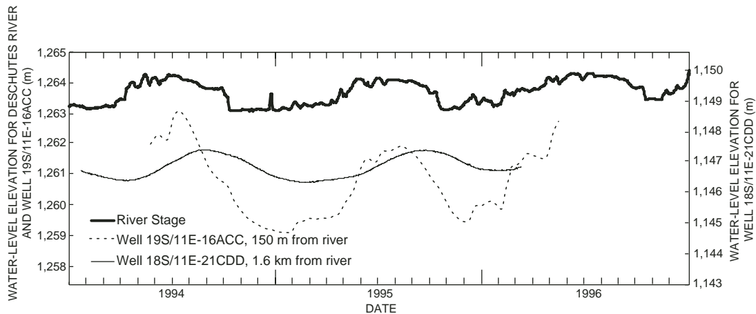
Figure 32. Hydrograph showing the relation between the stage of the Deschutes River at Benham Falls and water levels in wells 150 and 1600 m from the river. Modified from Gannett et al. (2001).
