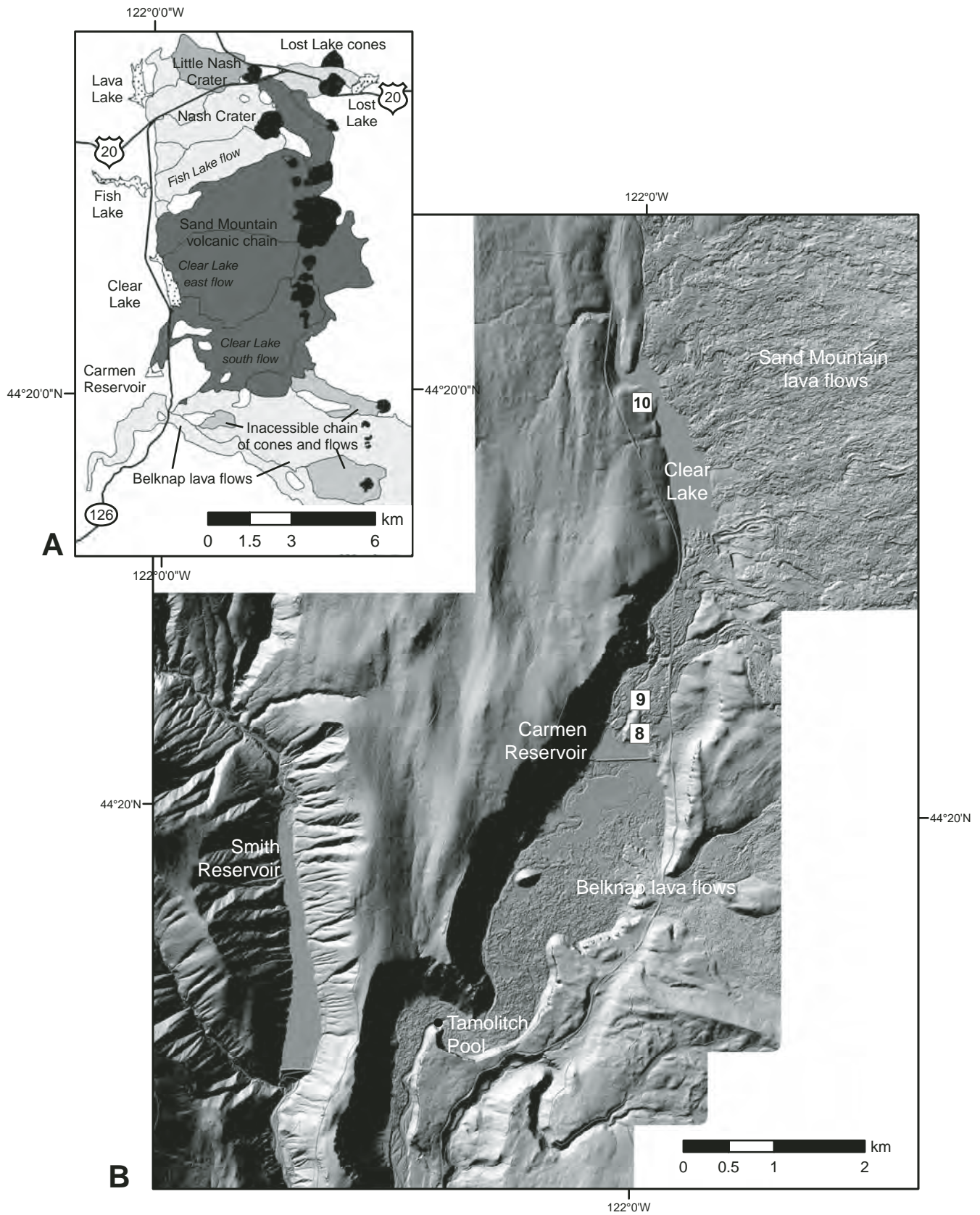
Figure 17. (A) Young lava flows (<math><4000\text{ }^{14}\text{C yr B.P.}</math>) that entered the McKenzie River Valley. Modern lakes and reservoirs are shown in light gray. Geology from Sherrod et al. (2004). (B) Light detection and ranging (LiDAR) of upper McKenzie River, with stop locations (squares) and Tamolitch pool (black dot) shown.
