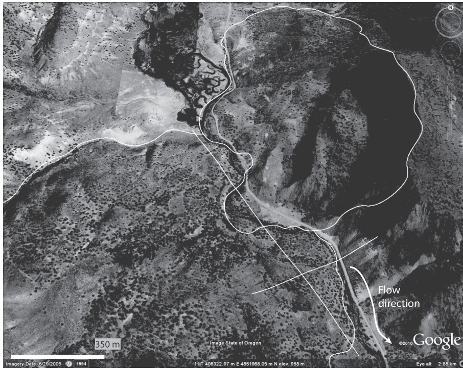
Fig. 9. Oblique Google Earth image of Chukar Park landslide dam site. North Fork Malheur River flows from top to bottom of image. A pair of landslide complexes, outlined in white, flank the river on both sides. Based on field observations, the landslide dam crest is believed to be along the short, valley-perpendicular line, and the breach zone is spanned by the long, valley-parallel line.
