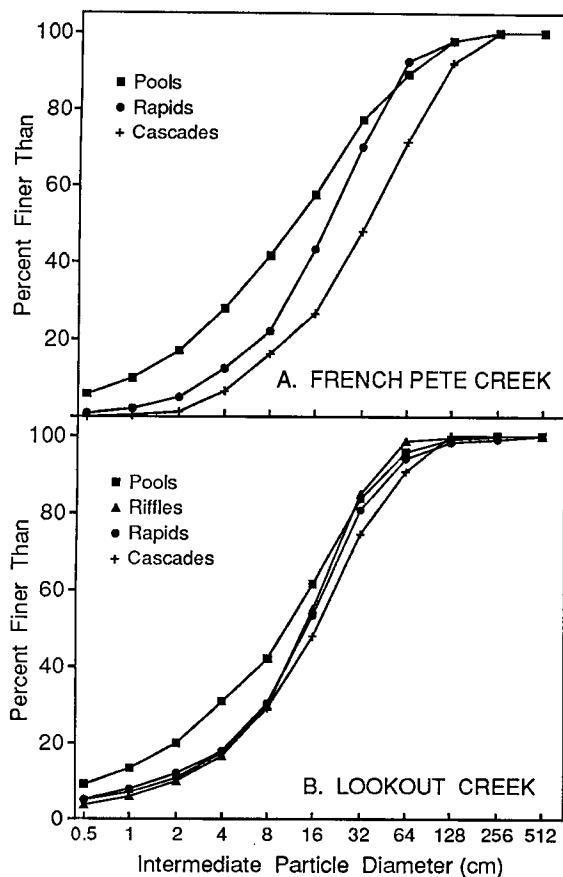
Figure 5. Particle size distribution for French Pete Creek (A) and Lookout Creek (B), based on counts of 750 and 1,200 particles, respectively.
