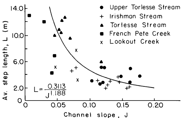
Figure 6. Average spacing between steps in rapids and cascades in relation to bed slope. Data points for French Pete and Lookout Creeks represent the average spacing of three to seven steps. Data points and curve for Torlesse and Irishman Streams (New Zealand) from Whittaker (1987a).
