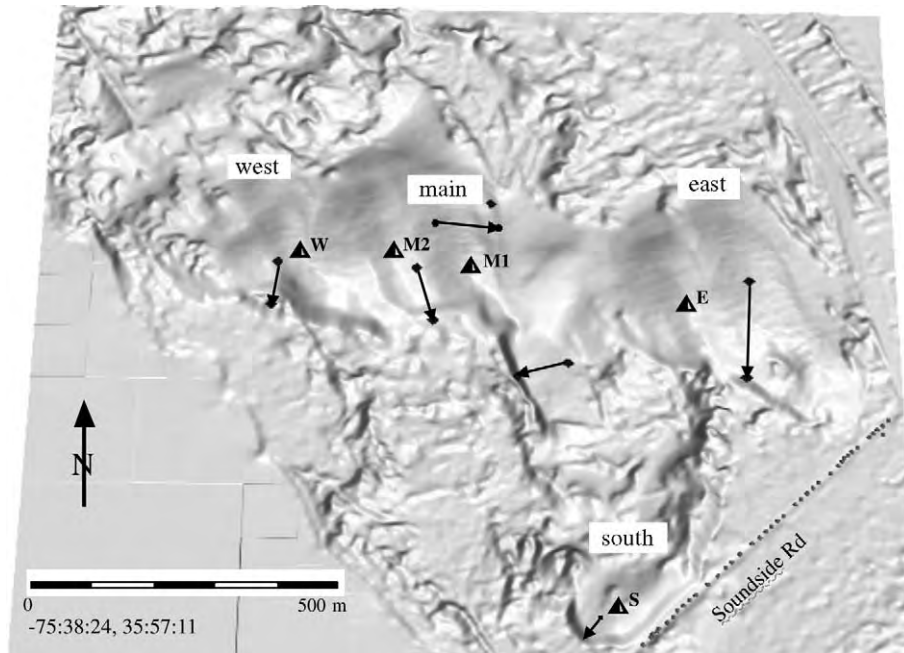
Fig. 2. Dune field elevation surface in 2001 showing location of individual dunes (main, south, east and west), their respective peaks (M1, M2, S, E, W), points on the Soundside Road used for accuracy testing, and representative profiles used for assessment of horizontal dune migration (arrows).
