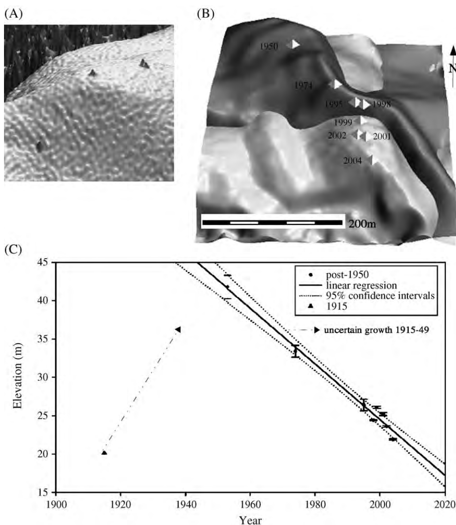
Fig. 5. Jockey's Ridge main dune peak: (A) noise or people captured near the top of the dune in 1999 lidar data; (B) peak migration 1953–2004 (1974: dark surface, 2001: light surface); (C) change in elevation 1915–2004.
