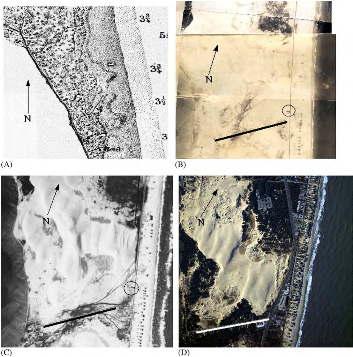
Fig. 9. Evolution of land cover: (A) 1879 nautical chart with portion of the study area covered by vegetation; (B) 1932 air photography (USACE FRF, 2004) showing no vegetation; (C) 1940 air photography with a small patch of low vegetation in a NE wet area; (D) 2003 air photography (post-hurricane Isabel) with the dune complex surrounded by dense vegetation.
