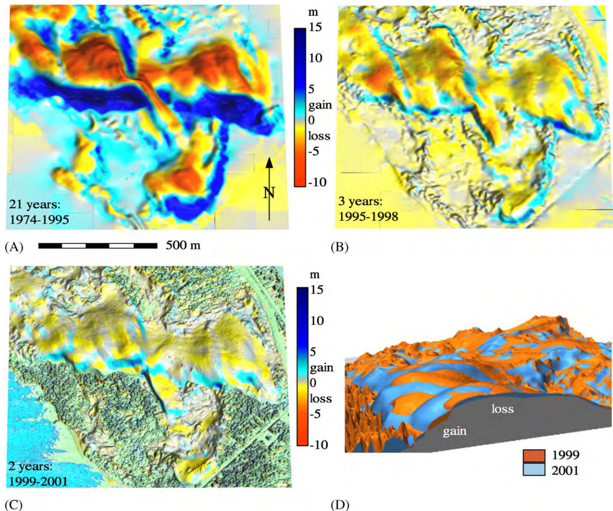
Fig. 8. Long-term and short-term elevation differences revealing continuing sand loss on the northern, windward side of the dunes and gain mostly on the southern side of the dunes along the slip faces: (A) 1974–1995; (B) 1995–1998; (C) 1999–2001; and (D) cross-section of the main dune showing dune flattening between 1999 and 2001 (profile is colored by the bottom surface).
