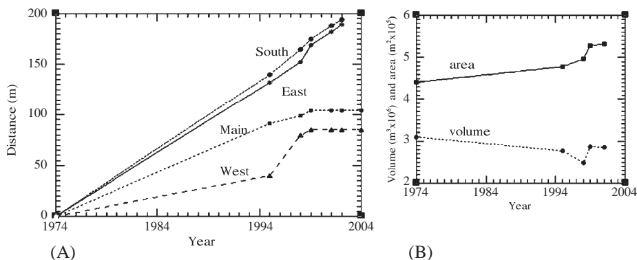
Fig. 6. Evolution of the dune field: (A) horizontal migration of individual dunes given as cumulative distance measured between the dune crests along representative profiles (see Fig. 2) and (B) dune volume and area change for the active dune subregion defined by elevation z > 6 \text{ m} .
