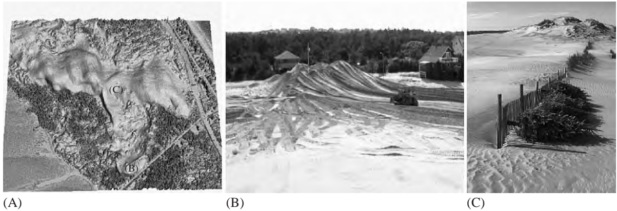
Fig. 10. Dune management: (A) location of recent management actions; (B) removal of south dune; (C) stabilization fences enhanced by discarded Christmas trees.
