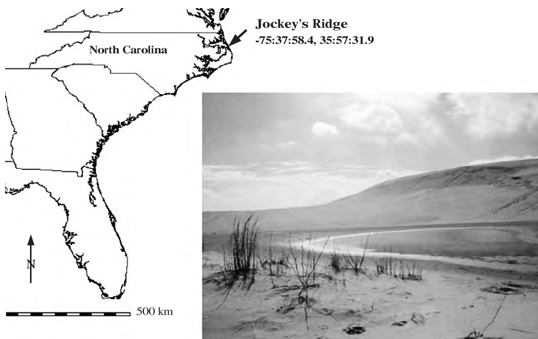
Fig. 1. Location of Jockey's Ridge dune field on the Outer Banks, the North Carolina barrier islands. Photo shows a view of the dune from the NE after rainfall in 2003.
