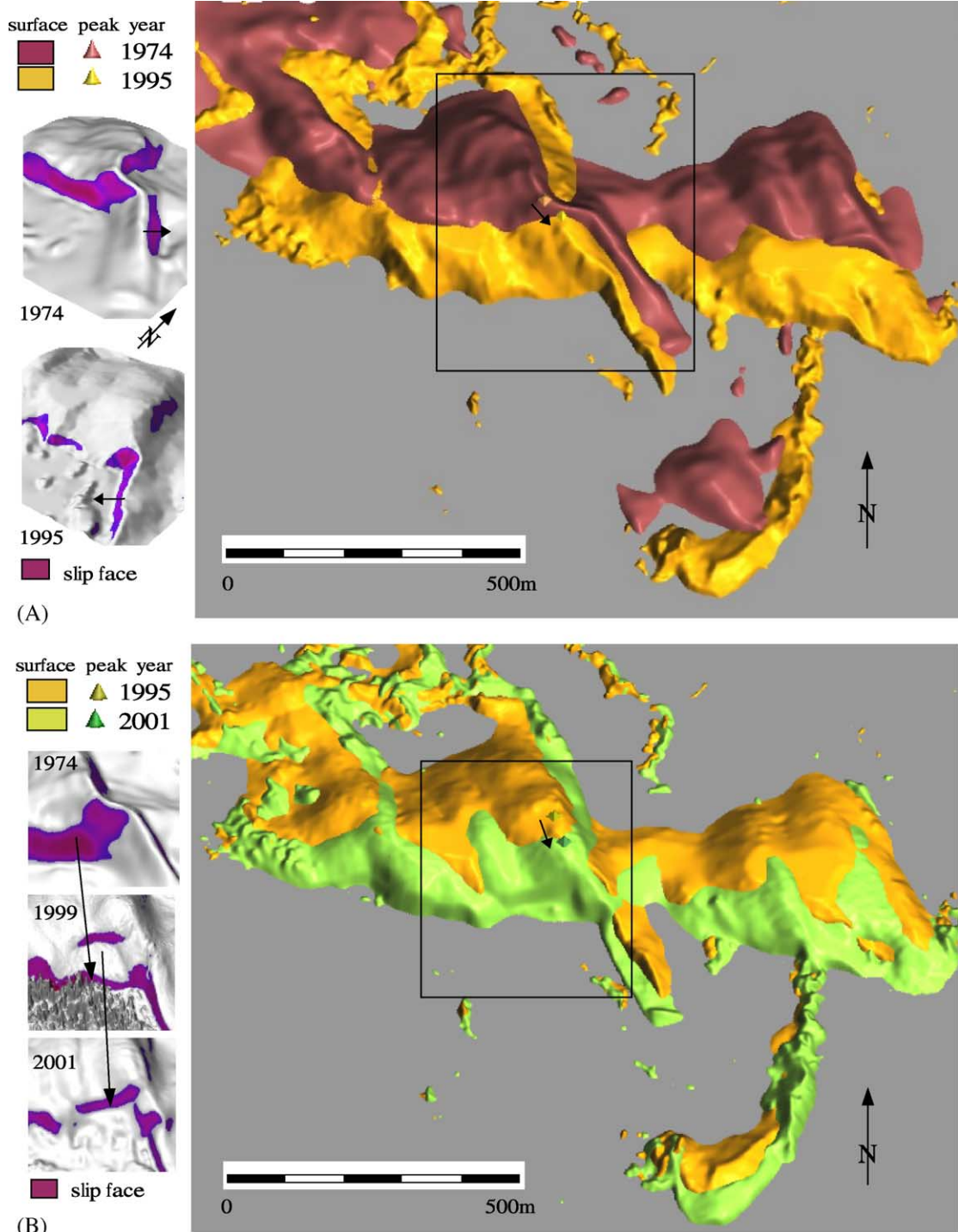
Fig. 7. Overlay of active dune surfaces (subregions without vegetation where elevation z > 6 m), demonstrating similar patterns of southward migration between (A) 1974–1995 and (B) 1995–2001. Higher of the two surfaces is visible and migration of the main peak is represented by arrow. Inserts show changes in slip faces: (A) reversal in the slip face direction from east in 1974 to west in 1995 on the lower ridge of the main dune and (B) evolution of a new slip face “inside” the main dune in 1999.
