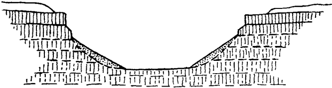
FIG. 10.—Devils Canyon, cross-section a mile and a half south of Kahlotus, showing (1) steepened loessial bluffs ( 33^\circ ), (2) narrow scabland above brink of basalt cliffs (3) canyon 450 feet deep and less than one-fourth mile wide, and (4) post-Spokane talus, three-fourths the height of the cliffs. Horizontal and vertical scale the same.
