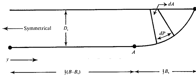
FIGURE 4. Definition diagram outlining assumed channel geometry of straight reaches of coarse-gravel rivers.
