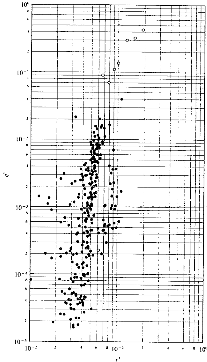
FIGURE 7. Bed load relation for gravel beds.
