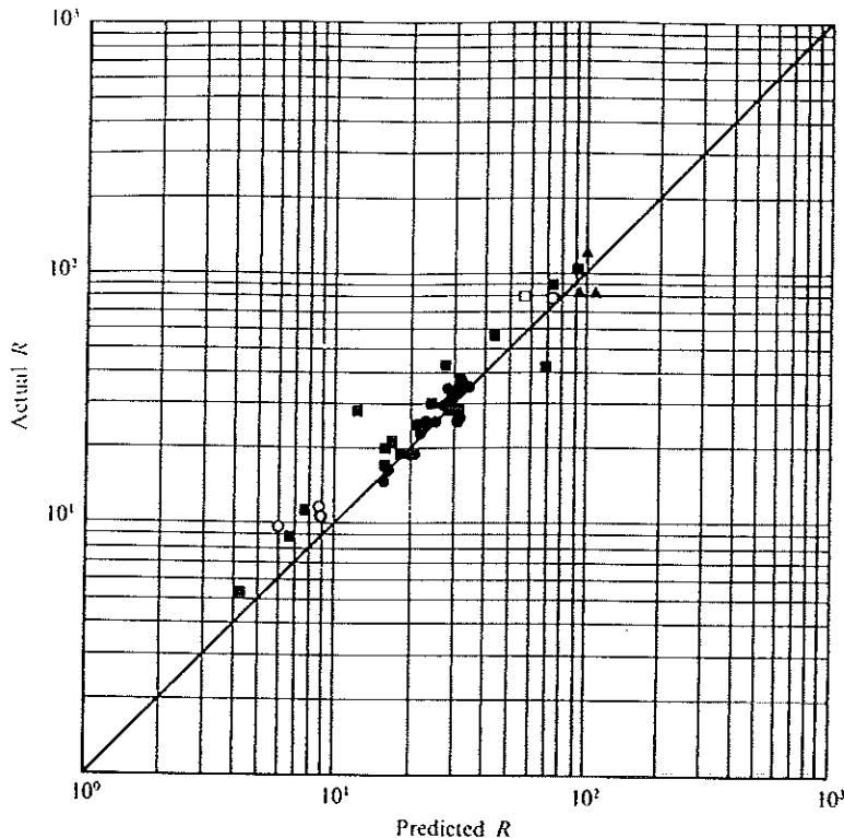
FIGURE 10. Test of the second regime relation (34). Calculated values of R are compared with observed values. Symbols as in figure 9.
