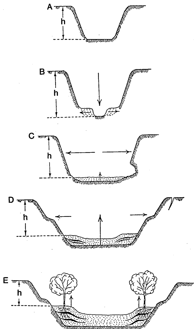
Figure 2. Evolution of incised channel from initial incision (A, B) and widening (C, D) to aggradation (D, E) and eventual relative stability (after Schumm et al., 1984); h is bank height.
