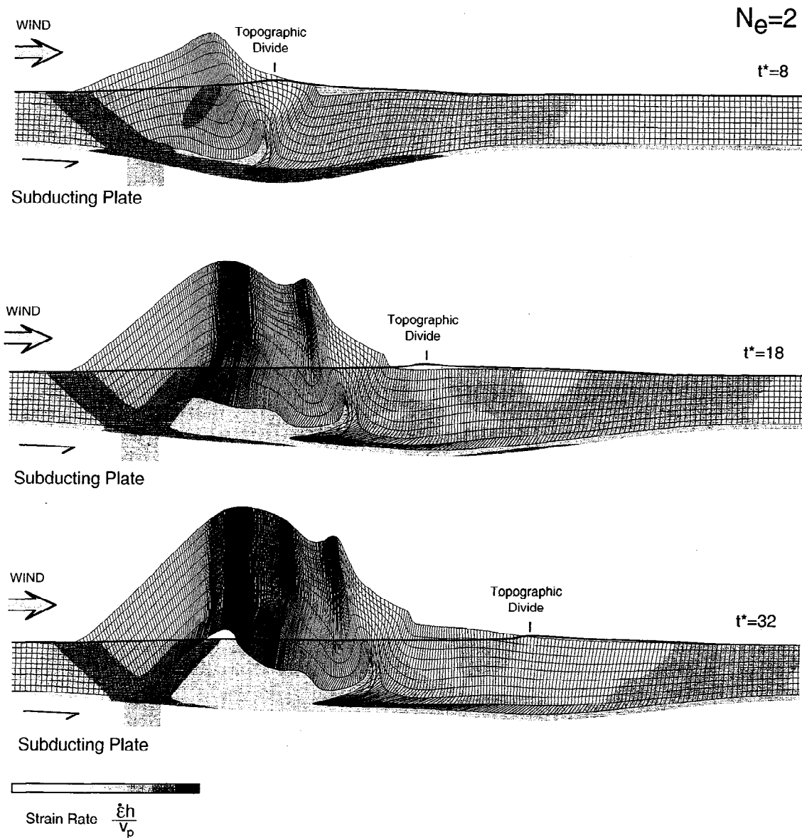
Figure 13. Model with precipitation focused on prowedge. Prowedge is characterized by an erosion number N_e of 2. Retrowedge has no erosion ( N_e = 0 ). Results are shown at nondimensional times t^* of 8, 18, and 32. Lower figure is near steady state. See Figure 3 caption for additional model description.
