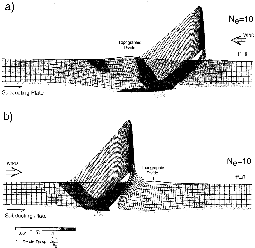
Figure 15. Model with orographic focusing of precipitation at high erosion number ( N_e=10 ): (a) precipitation and erosion focused on retrowedge, and (b) precipitation and erosion focused on prowedge. Results are shown at nondimensional time t^* of 8 which is at steady state. Note similar patterns of exhumation but offset relative to topography. See Figure 3 caption for additional model description.
