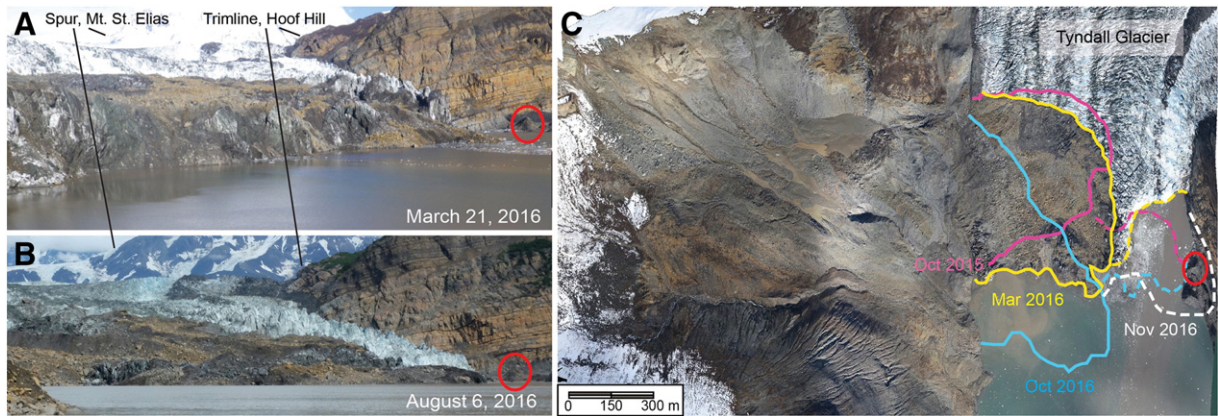
Fig. 15. Oblique photographs and time series of the changes at the terminus of Tyndall Glacier on (A) 21 March 2016 and (B) 6 August 2016. Note lowering of the ice surface in (B) and advection of the supraglacial landslide debris to the waterline. Red circles indicate the location of the largest hummock proximal to the ice front. (C) Outlines of the locations of supraglacial landslide debris from October 2015 until November 2016. The underlying image was taken in March 2016.
