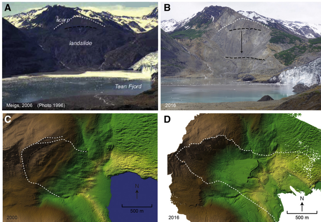
Fig. 3. (A) The slope in 1996 (from Meigs et al., 2006) already displays signs of sliding. (B) The same view after the 2015 catastrophic failure (image taken in June 2016). (C) and (D) are DEMs before (2000) and after (2016) the catastrophic failure. (C) Precursory slope deformations are discernible in the form of backscarps. (D) The large volume excavated from the source area, change in shore line and in the glacier terminus after loading by landslide debris are apparent.
