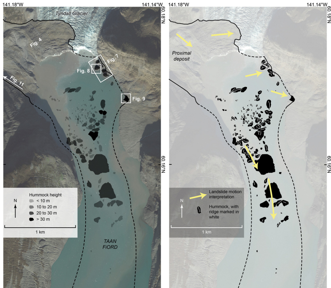
Fig. 6. Distribution map of hummocks based on lidar images and bathymetry data. The left panel shows hummock area and height, the right panel includes hummock ridges (white lines) and indicates landslide spreading direction based on hummock alignments, geomorphometry, and structural data. The two large hummocks downfjord are compound landforms. Solid lines are known landslide deposit boundaries, dashed lines infer this boundary.
