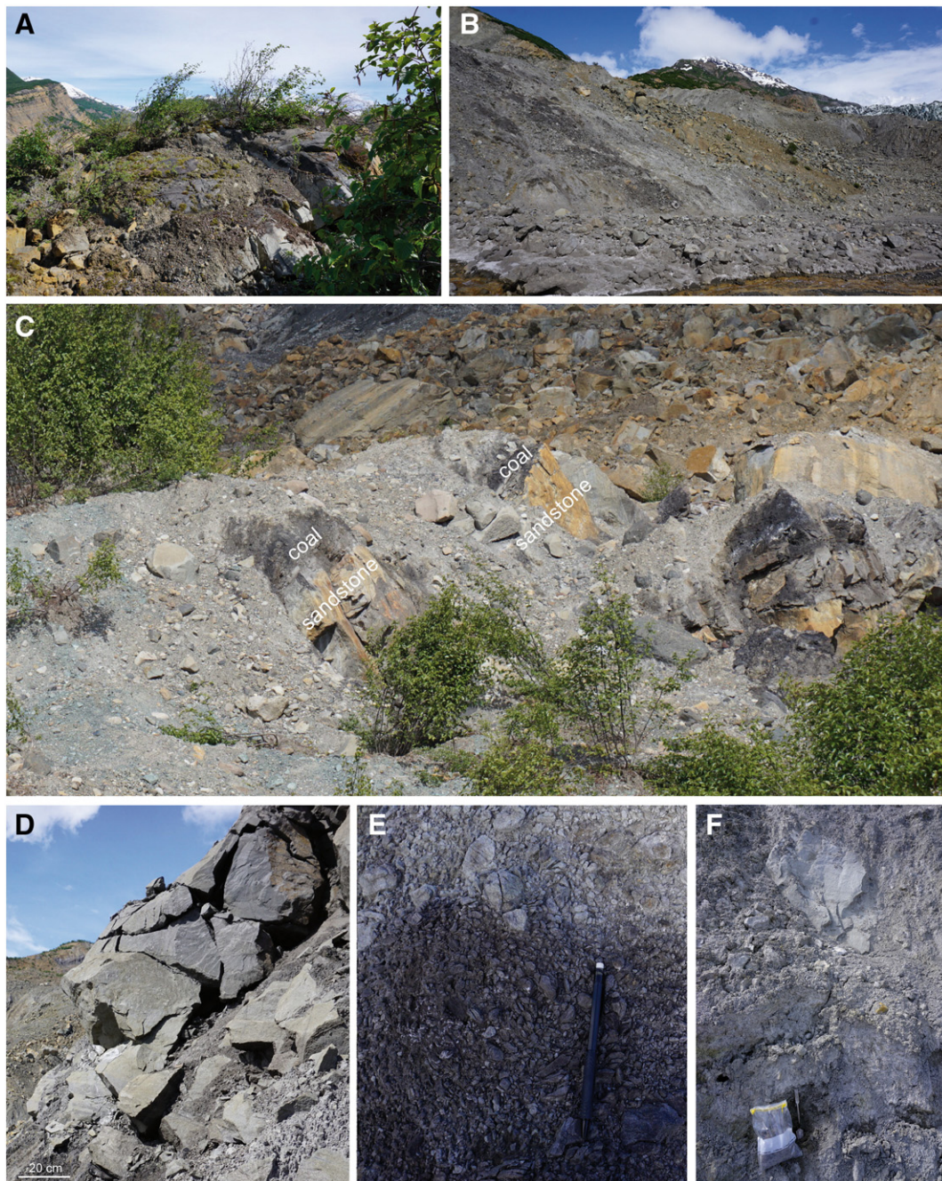
Fig. 4. (A) Glacial-polish on megablocks on top of slide block. (B) Coloured bands on the landslide surface are a function of rock type, weathering coat, and grain size (compare to Fig. 5). (C) Preserved layers in slide block debris. (D) In-situ fractured (= jigsaw-fractured) block. (E–F) Fragmented facies.
