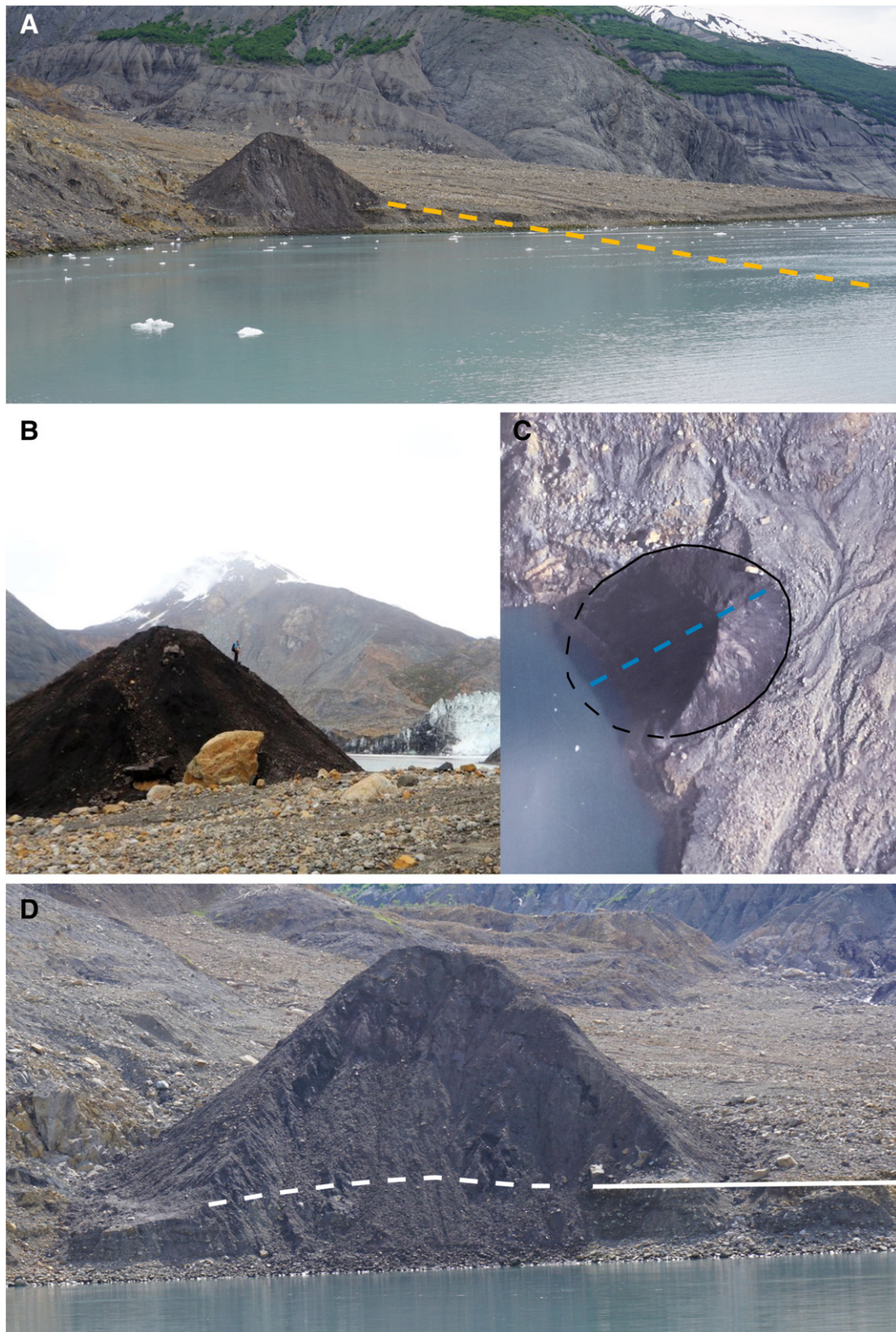
Fig. 9. Distal hummock on Hoof Hill fan. (A) Path of re-emergence after travel through the fjord water to the final deposition site on land. (B) View from Hoof Hill fan toward the landslide failure scarp with person for scale. (C) Reconstruction of hummock shape and long axis orientation; long axis length (dashed blue line) is 75 m. (D) The solid white line traces the original fan surface beneath the distal hummock and the dashed white line traces the elevation of entrained pebbles. See Fig. 6 for location.
