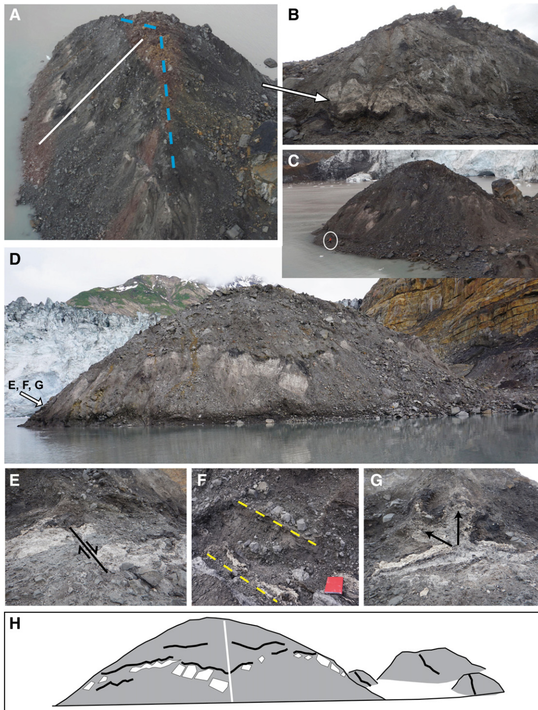
Fig. 8. Deformation features within one of the subaerial hummocks (A–D) and the gouge material at its base (E–G). Blue dashed line (A) traces ridge lines (compare to Fig. 6); white lines (A, H) connect the bend in ridge axis with structural features in the interior. White circle (C): person for scale. Tilted layers (D), offset gouge (E), shear band (lower yellow line) parallel to aligned clast (upper yellow line; F), (G) diapir of gouge material. (H) is a simplified sketch of the hummock in (D) showing sub-horizontal layers in the large and sub-vertical layers in the small hummocks (black: coal layers; white: faulted sandstone unit); motion direction is roughly left to right (D, H). See Fig. 6 for location.
