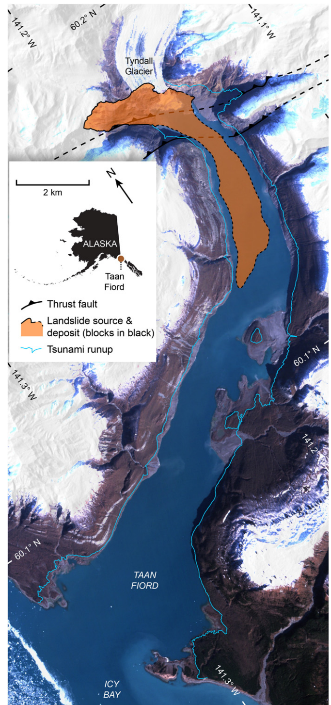
Fig. 1. Setting of the 17 Oct 2015 Taan Fiord Landslide and Tsunami. The source rocks lie north of two faults that divide the Yakataga formation in the south, from the Kulthieth formation in the north. The sliver of crust between the faults has been most recently mapped as Yakataga (Chapman et al., 2012).
