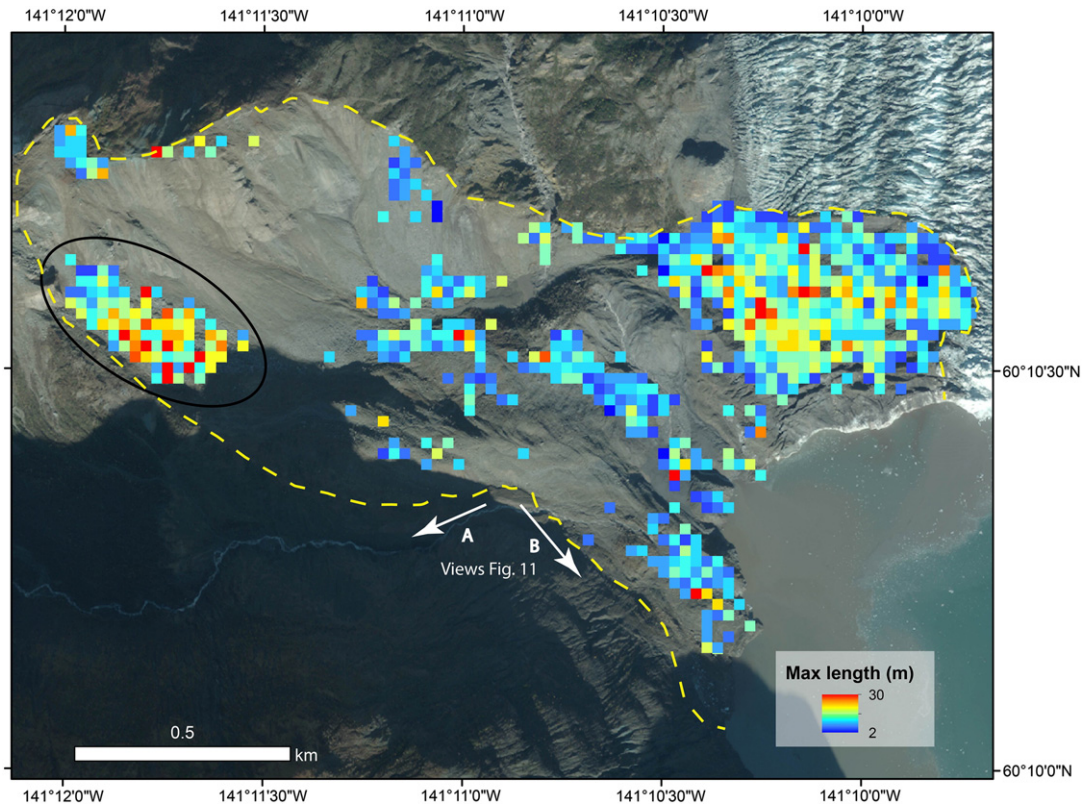
Fig. 12. Neighbourhood analysis of boulder size for the source area and supraglacial landslide deposit; the extent of the 2015 landslide deposit is marked by yellow dashed line. Coloured squares represent 625 m 2 squares, and the largest boulder in each is mapped. The boulders inside the black circle belong to a separate, later rockfall event.
