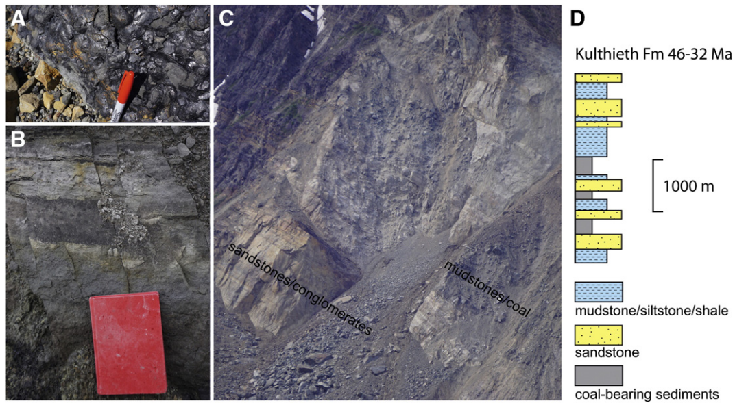
Fig. 2. (A) Sandstone clast with coal layer, and (B) mudstone clast in the landslide debris. (C) Overview of the uppermost landslide scarp of 2015 (section is roughly 300 m high and is a close-up of the area in the top left corner above the 1996 scarp (white dashed line) in Fig. 3B). (D) Stratigraphy of the Kulthieth Formation (after Pavlis et al. (2012) and van Avendonck et al. (2013)). The profile is from the hanging wall of the Chaix Hill fault and thus, within Taan Fiord the Kulthieth Fm. does not exist in its full thickness.
