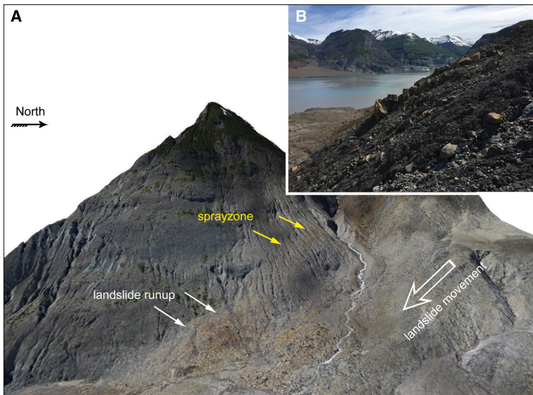
Fig. 11. (A) Landslide traces beneath Daisy Glacier valley. (B) Field photo of scattered angular boulders taken from the area just below the two yellow arrows (spray zone) shows landslide debris draped over the slope. See Figs. 6 and 12 for location.
