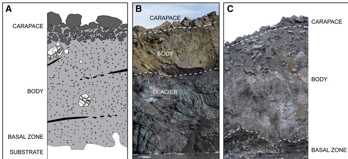
Fig. 17. (A) Sketch of the typical three-part depositional facies model of large landslides; not to scale. The equivalent facies in the Taan landslide: (B) supraglacial debris (ice thickness above waterline is roughly 10 m; the boundary to overlying landslide debris is not clear since some areas of landslide debris look ice-cored with only a thin layer of fines draped over the cliff, hence the presence of a basal zone cannot be verified), and (C) hummock on land (compare to Fig. 8).
