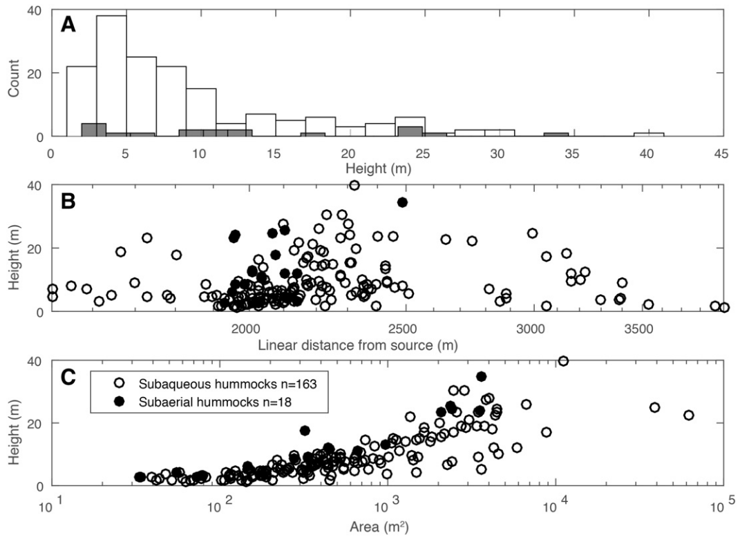
Fig. 10. Statistics of hummock size and travel distance. (A) Histogram of hummock heights. (B) Scatterplot of hummock height and linear travel distance from common point in source area (see Fig. 9); as distances are straight-line, they should be treated as minima. (C) Scatterplot of area and height. All panels differentiate between subaerial and subaqueous hummocks. Note that many of the subaqueous hummocks are partly buried by fine sediment that has settled since the landslide occurred. As a result, those measurements should be treated as minima.
