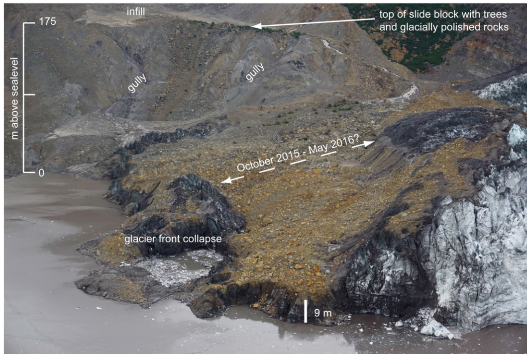
Fig. 16. This photograph from May 2016 shows the rapid denudation of the glacier terminus, erosion of the landslide debris (gullies in the slide block and supraglacial debris advected into the fjord), and stretching of the glacier in response to landslide loading.
