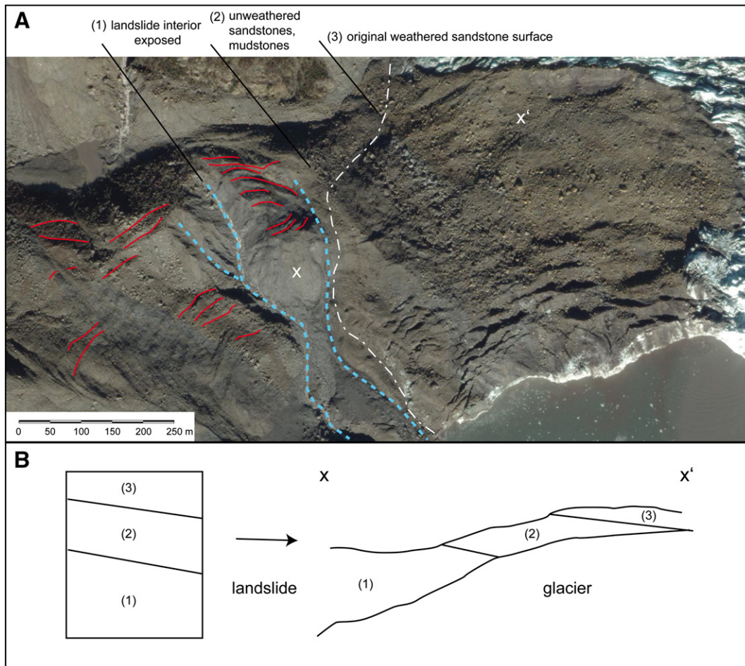
Fig. 5. (A) Aerial view of the supraglacial landslide deposit and the slumped debris within the source area; red lines are slumps/normal faults, blue lines are active fluvial channels eroding deep gullies into the debris, and the white dashed-dotted line traces the approximate margin of Tyndall Glacier. (B) Conceptual sketch as a potential explanation for the striped appearance of the debris along a virtual profile x-x' .
