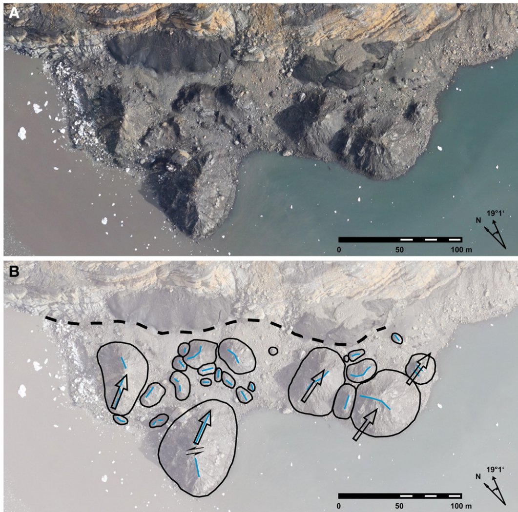
Fig. 7. Hummocks on land (east of the glacier, Fig. 3B) outlined in black; blue lines are ridge crests and the arrows show motion direction of the debris deduced from geomorphometric and structural data. Dashed line shows the deposit margin against the cliff bottom and dead ice mounds (dark shaded areas in contact to the cliff). See Fig. 6 for location.
