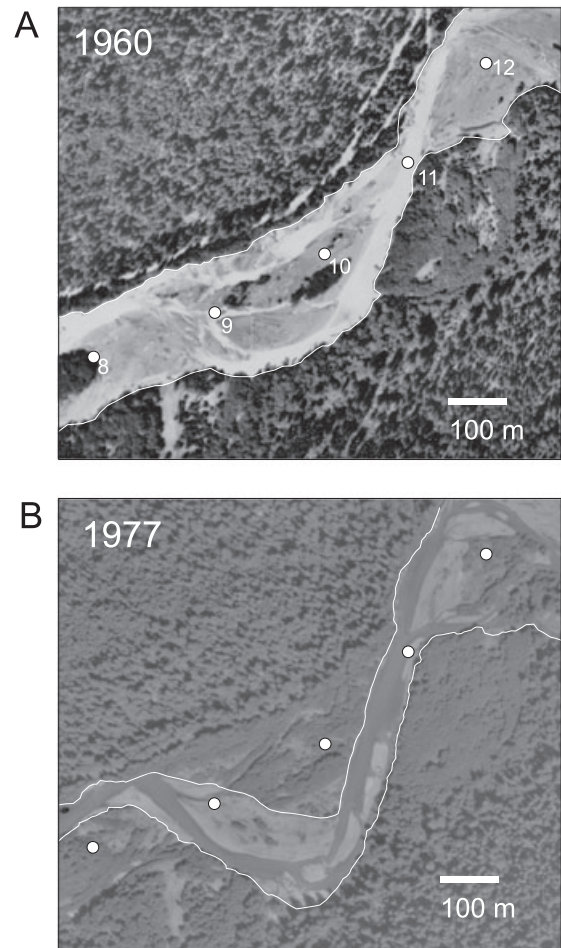
Figure 6. Photographs of the Hoh River study reach showing narrowing and simplification (decreased braiding) between (A) 1960 and (B) 1977. White circles show points corresponding to transects 8–12 (Figure 2(A)); circles indicate approximate center of active river corridor as of 2013.
