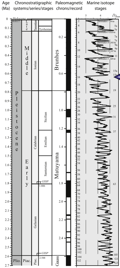
Modified from Cohen and Gibbard (2010)
