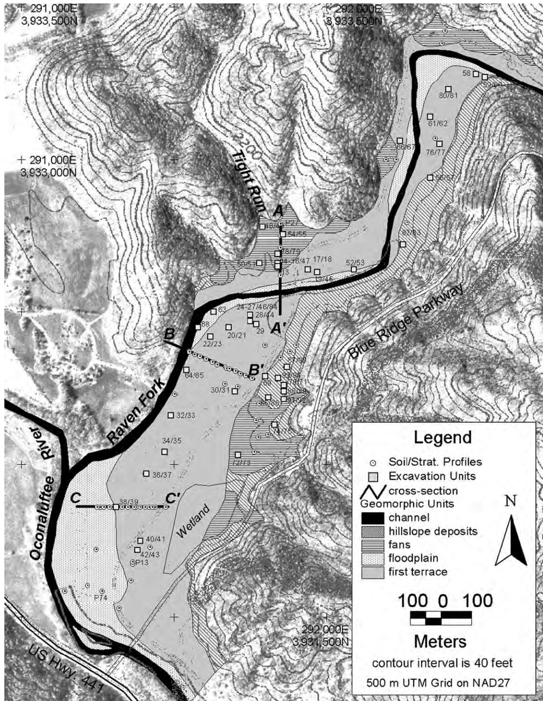
Fig. 2. Geomorphic map of the lower Raven Fork stream valley at its confluence with the Oconaluftee River, including topographic lines from the Smokemont, 7.5-min USGS quadrangle. The north and west side of Raven Fork is part of the Great Smoky Mountains National Park and the south and east side includes the Qualla Cherokee Reservation as well as additional park land.
