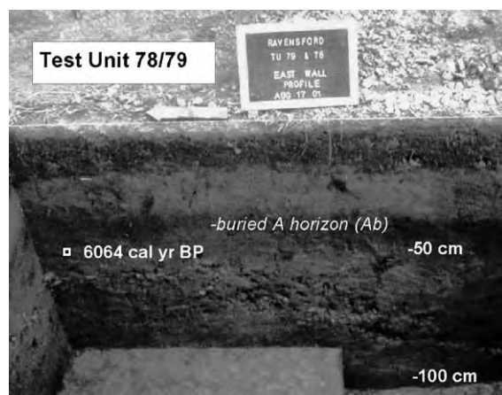
Fig. 5. Photograph of typical alluvial/colluvial fan deposits.
