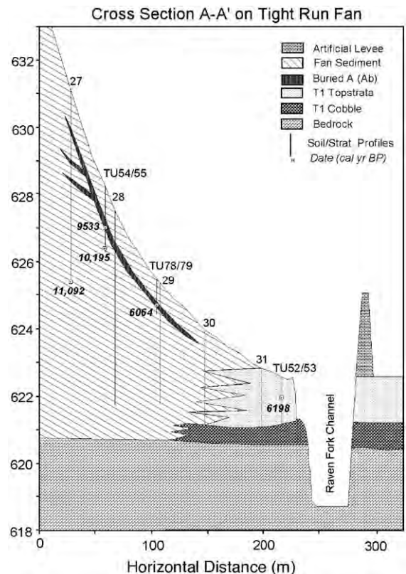
Fig. 4. Longitudinal stratigraphic cross-section through the Tight Run alluvial fan (A–A' on Fig. 2).
