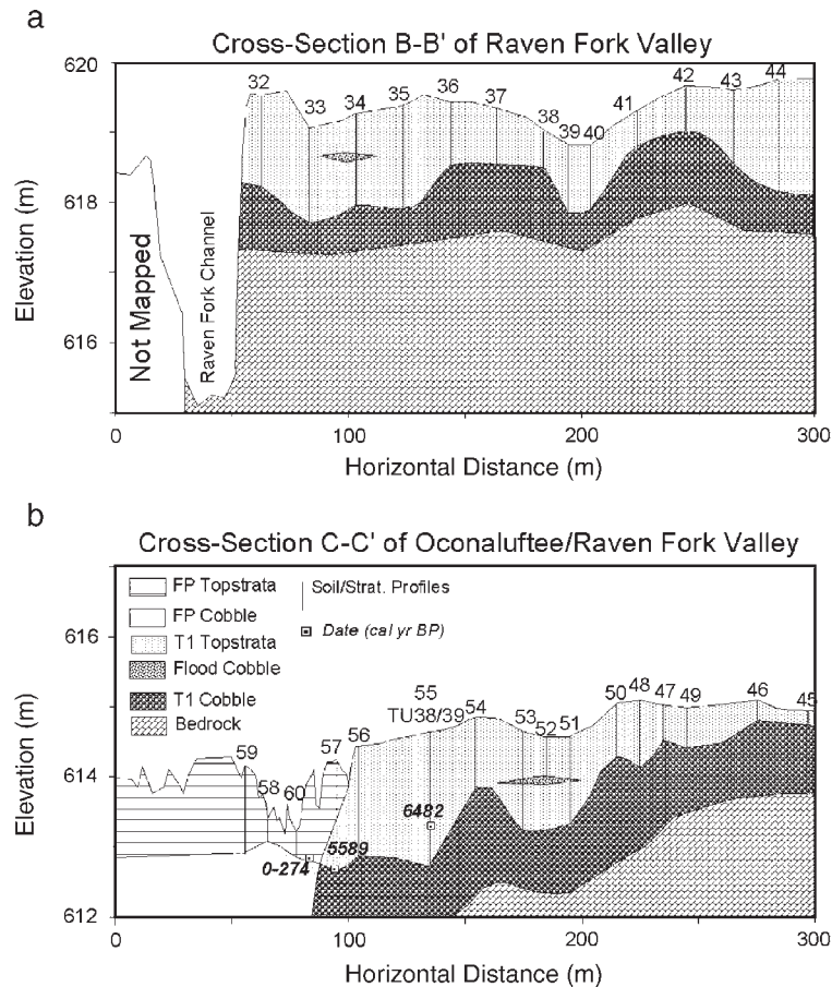
Fig. 6. Transverse stratigraphic cross-sections of the floodplain and terraces looking upstream through B–B' (6a) and C–C' (6b) on Fig. 2.
