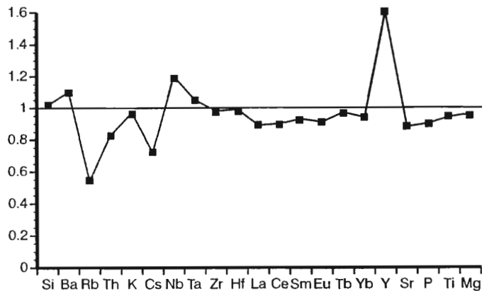
Figure 16. Clast from a pyroclastic-flow deposit of Old Maid age (63.7 percent \text{SiO}_2 ; analysis 3) normalized to a clast from a diamict of Polallie age (62.5 percent \text{SiO}_2 ; analysis 7).
