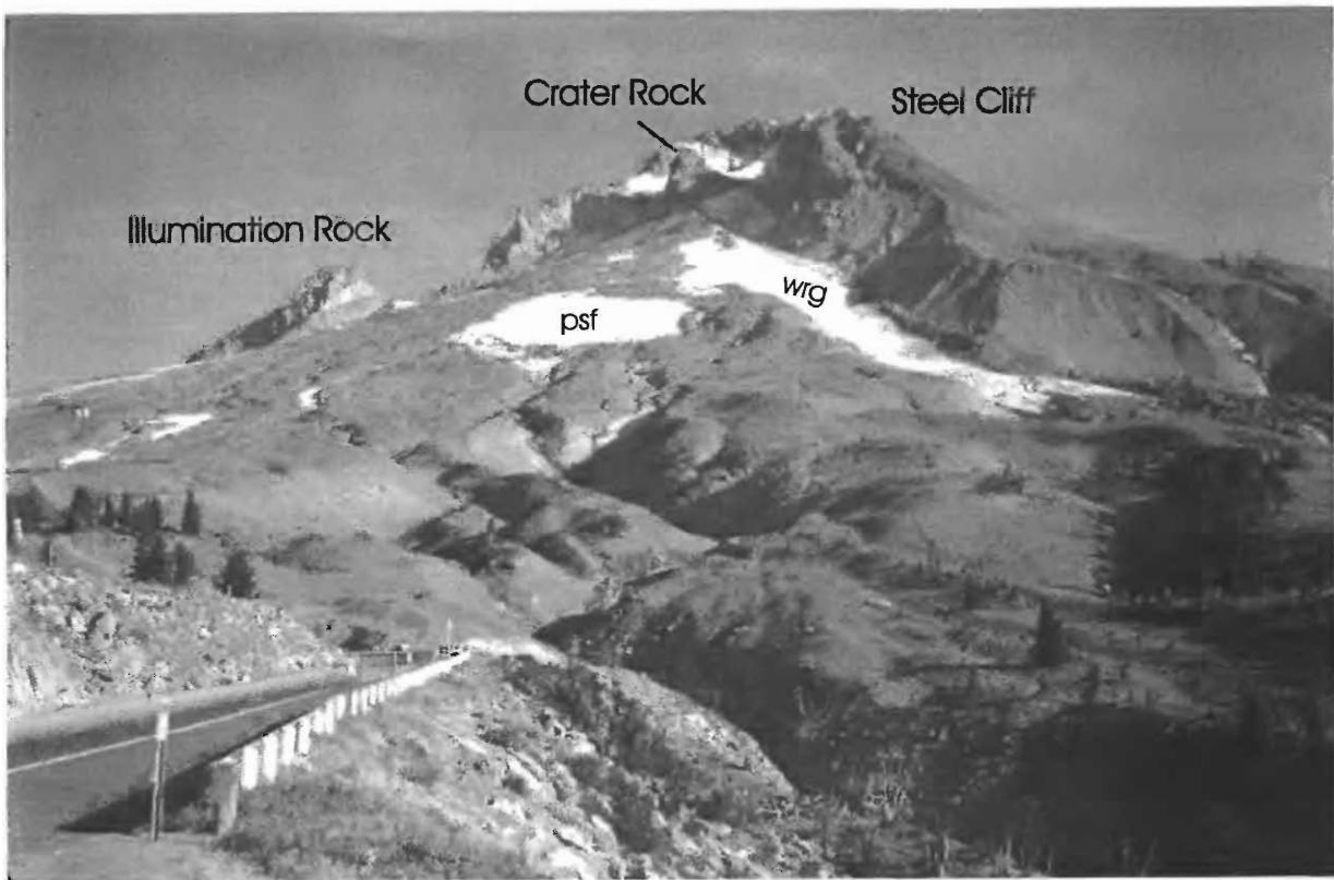
Figure 17. Photograph of upper south flank of Mount Hood from Stop 8 showing prominent summit features and broad fan of pyroclastic-flow and lahar deposits. psf , Palmer Glacier (snowfield); wrg , White River Glacier. Surface from psf to center left is chiefly Timberline age and surface extending to right of terminus of wrg is underlain by deposits of Old Maid age. Gullies and rolling surface in center to lower right is underlain by deposits of Polallie age, as is surface that extends to right center below Steel Cliff. Andesite lava flow is exposed in roadcut and slope below road.
