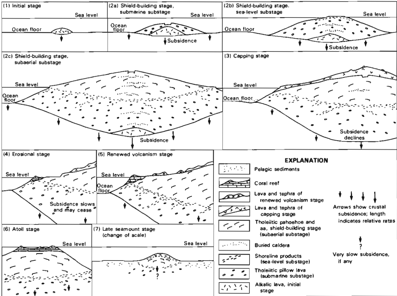
FIGURE 7.9.—Diagrams showing successive stages in evolution of a Hawaiian volcano as proposed in this paper. Changes between stages normally are transitional and gradational. For simplicity, feeder conduits and rift zones are omitted. Substantial crustal subsidence caused by volcanic loading occurs throughout growth stages (1) through (3); subsequent sea-level changes may be sporadic, but net subsidence continues into stage (7). Vertical exaggeration varies from approximately 2× to approximately 4×. Only stages (1) through (4) are represented on Hawaii. See text for additional details.
