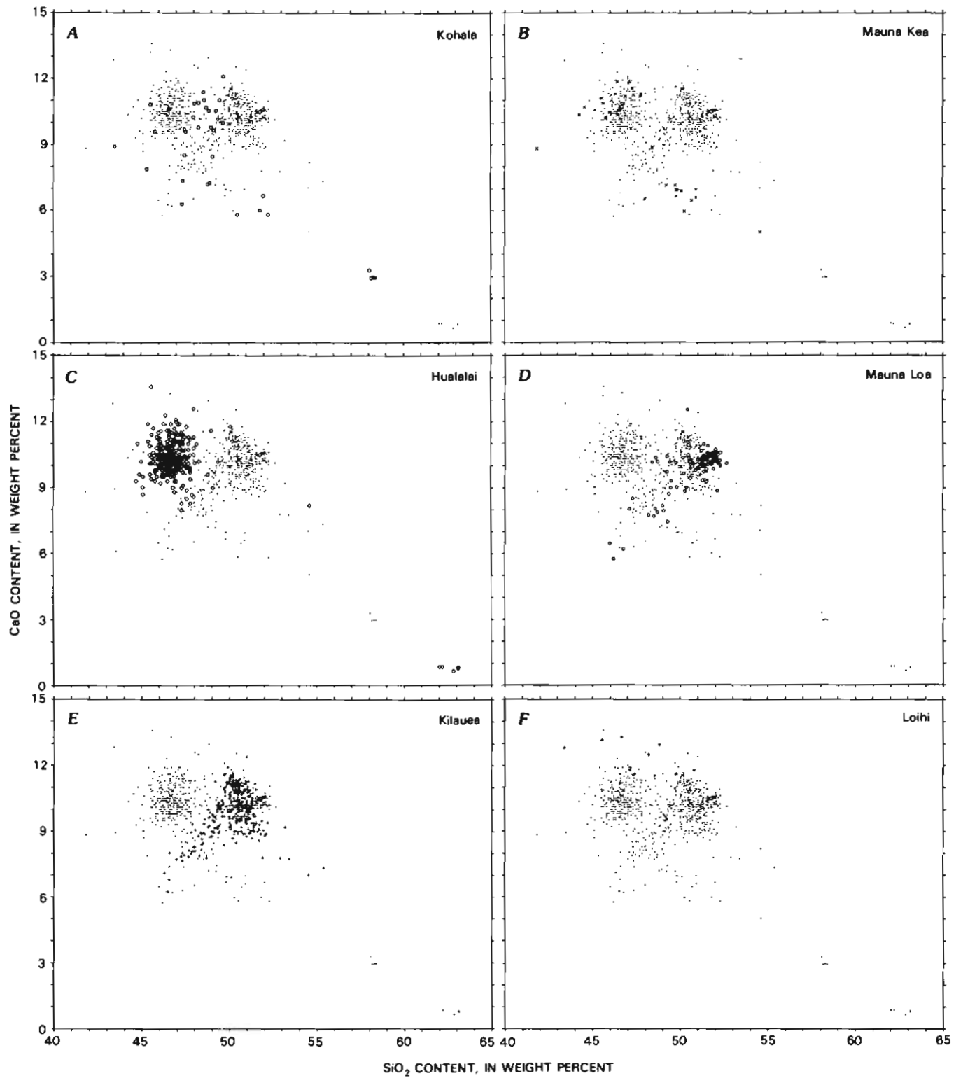
FIGURE 7.11.—Lime-silica variation diagrams (CaO vs. SiO 2 ) for volcanic rocks of Hawaii. A–F, Plots for individual volcanoes, as indicated. G, Data for all six volcanoes combined. Individual diagrams show data for that volcano by heavy symbols and for comparison data for other volcanoes by light dots. Analyses from published and unpublished sources.
