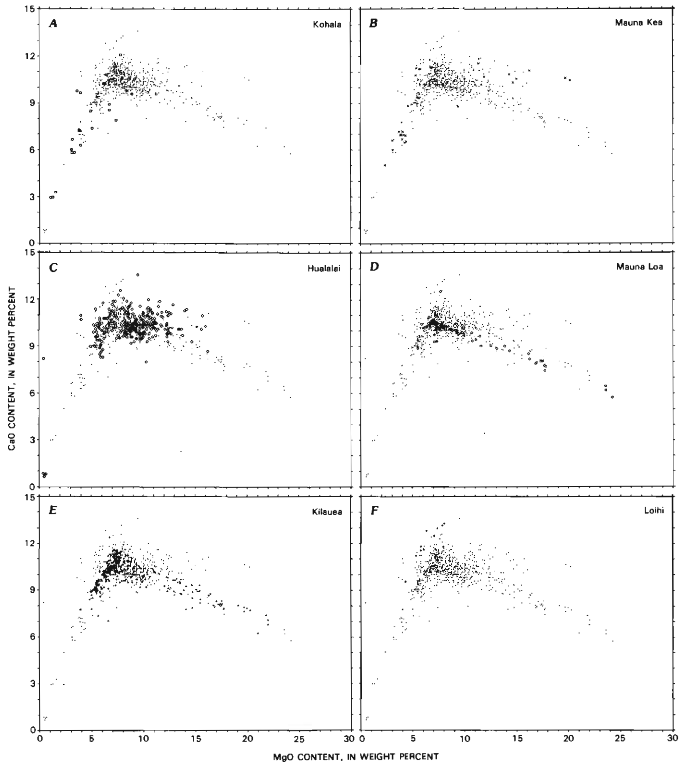
FIGURE 7.12.—Lime-magnesia variation diagrams (CaO vs. MgO) for volcanic rocks of Hawaii. A–F , Plots for individual volcanoes, as indicated. G , Data for all six volcanoes combined. Individual diagrams show data for that volcano by heavy symbols and for comparison data for other volcanoes by light dots. Analyses from published and unpublished sources.
