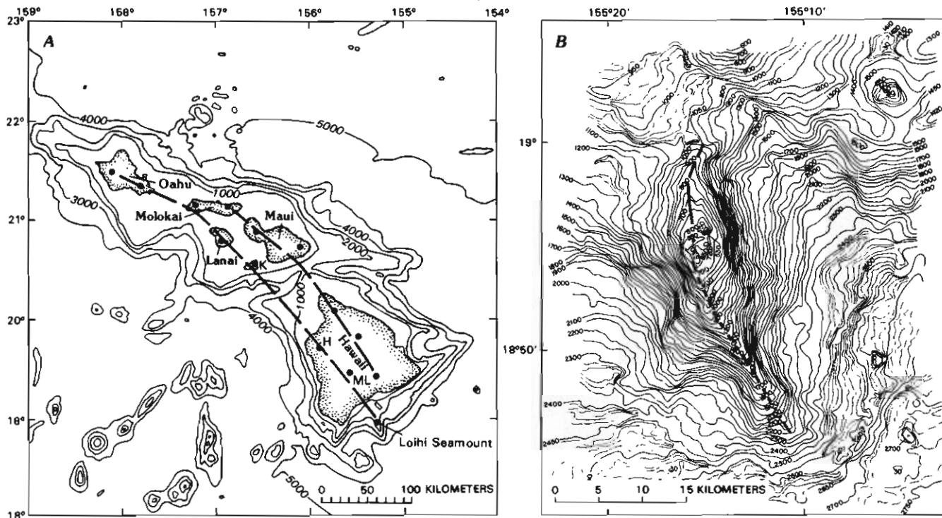
FIGURE 7.8.—Loihi Seamount. A , Position along regional curved locus extending through western line of volcanoes from Oahu to Hawaii, including Hualalai and Mauna Loa Volcanoes (after Moore and others, 1982). Bathymetric contours in meters. B , Bathymetric map (after Malahoff and others, 1982). Elongate ridges extending south-southeast and north from summit are major rift zones of volcano. They lie subparallel to volcano locus shown in A instead of parallel to submarine contours of island platform. Depth contours in fathoms (1 fathom = 1.83 m).
