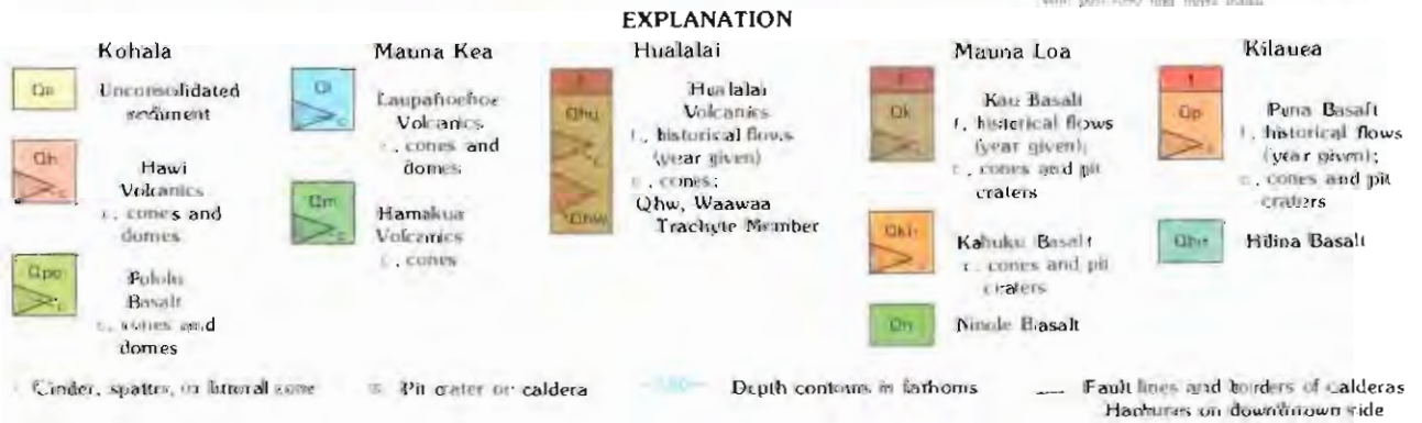
Geology from Stearns and Macdonald (1946) with post-1946 lava flows added.
