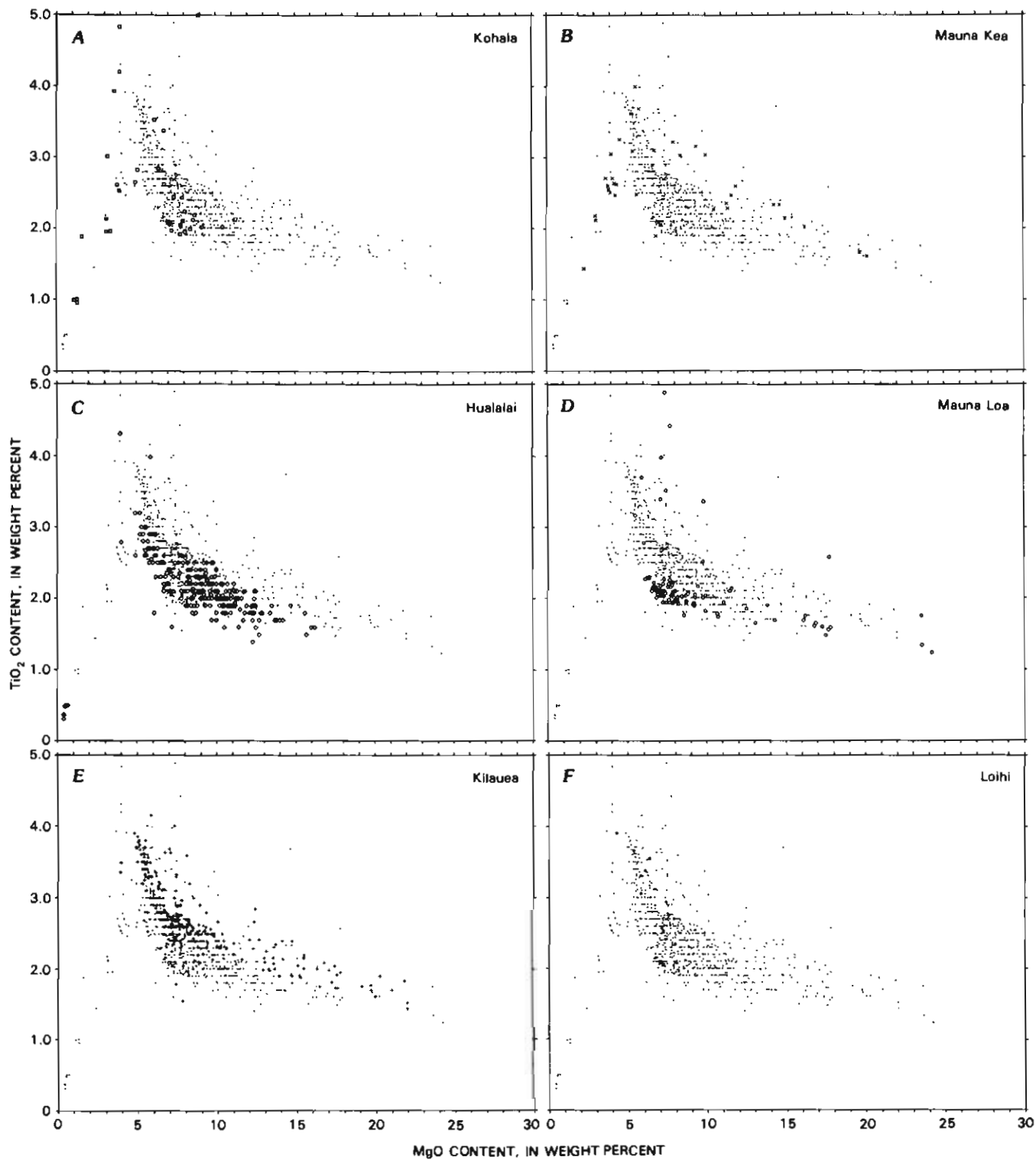
FIGURE 7.13.—Titania-magnesia variation diagrams ( \text{TiO}_2 vs. \text{MgO} ) for volcanic rocks of Hawaii. A–F , Plots for individual volcanoes as indicated. G , Data for all six volcanoes combined. Individual diagrams show data for that volcano by heavy symbols and for comparison data for volcanoes by light dots. Analyses from published and unpublished sources.
