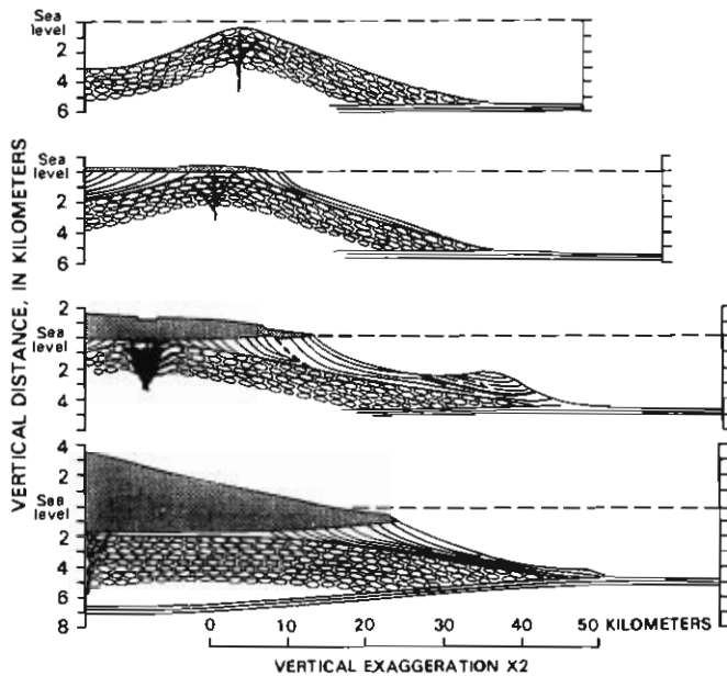
FIGURE 7.6.—Cross sections illustrating oceanic volcanic islands in submarine, sea-level, and subaerial stages of evolution (reproduced from Moore and Fiske, 1969, fig. 3, p. 1200). Patterns indicate rock types: ovals, pillow lavas with included pillow fragments and sediment; lined pattern, clastic rocks, including phreatic-explosion ash, littoral-cone ash, and flow-foot breccia and including some pillowed flows and pillow breccias; dark pattern, subaerial lava flows with minor ash; solid black, intrusive rock. Note contrast between submarine and subaerial slopes, continuation of clastic layer beneath subaerial shield, and downbowing of sea floor by subsidence caused by volcanic loading. Depth and elevation figures left side are in feet.
