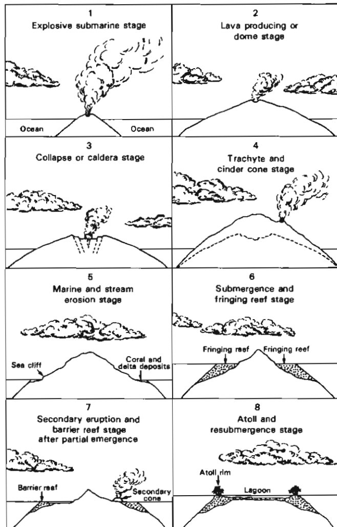
FIGURE 7.5.—Eight stages proposed by Stearns (1946) for geologic history of a volcanic island in the central Pacific.
