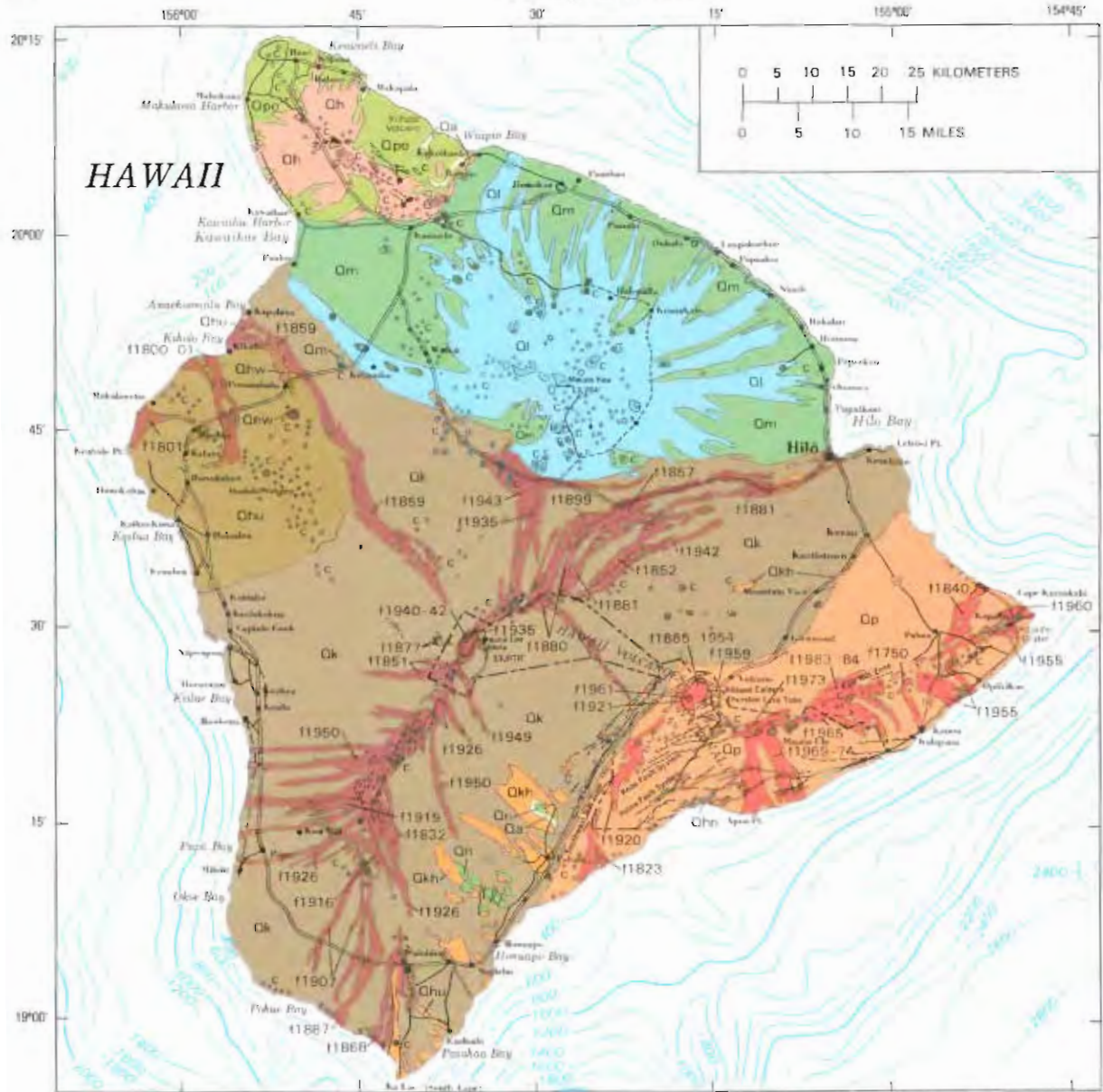
Geology from Stearns and Macdonald (1946) with post-1946 lava flows added.
