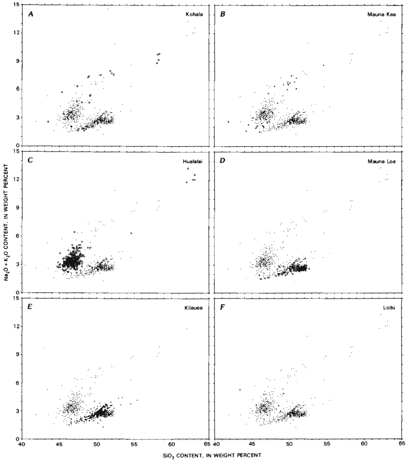
FIGURE 7.10.—Alkali-silica variation diagrams ( \text{Na}_2\text{O} + \text{K}_2\text{O} vs. \text{SiO}_2 ) for volcanic rocks of Hawaii. A-F , Plots for individual volcanoes as indicated. G , Data for all six volcanoes combined. Individual diagrams show data for that volcano by heavy symbols and for comparison data for the other volcanoes by light dots. Analyses from published and unpublished sources.
