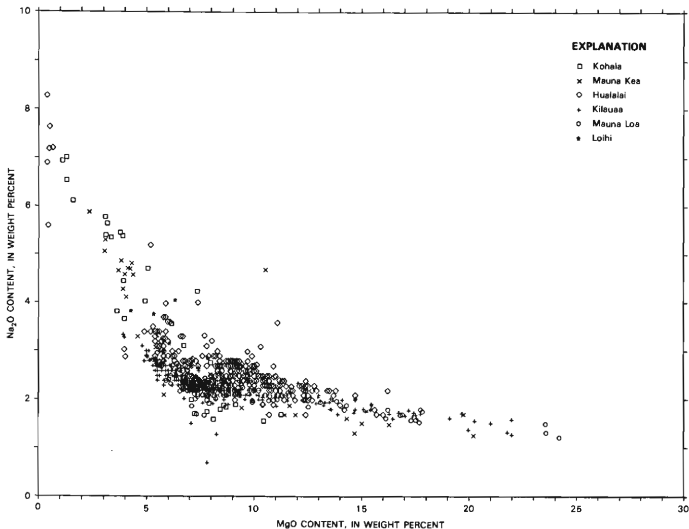
FIGURE 7.14.—Soda-magnesia variation diagram ( \text{Na}_2\text{O} vs. \text{MgO} ) for volcanic rocks of Hawaii. Analyses from published and unpublished sources.
