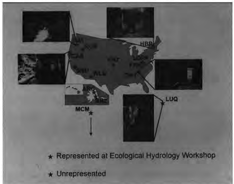
Fig. 1. Sites spanning a range of biome types and hydroclimatological regimes where long-term ecological and hydrologic research has been under way for as long as 6 decades. LTER sites represented at the ecological hydrology workshop (red stars) include the H. J. Andrews (HJA) conifer forest, Coweeta (CWT) deciduous forest, Hubbard Brook (HBR) mixed-conifer forest, Luquillo (LUQ) tropical rainforest, Arctic Tundra (ARC), McMurdo Antarctic Dry Valleys (MCM), Bonanza Creek (BNZ) boreal forest, and Konza Prairie (KNZ). Non-LTER sites represented include the Caspar Creek (CAS) U.S. Forest Service conifer forest and Reynolds Creek (RCR) U.S. Department of Agriculture rangeland site. Other sites with appropriate ongoing work that were not represented at the workshop (blue stars) but are involved in the study are San Dimas (SND), Walnut Gulch (WLG), Fernow (FRN), and Leading Ridge (LDR). Original color image appears at the back of this volume.
