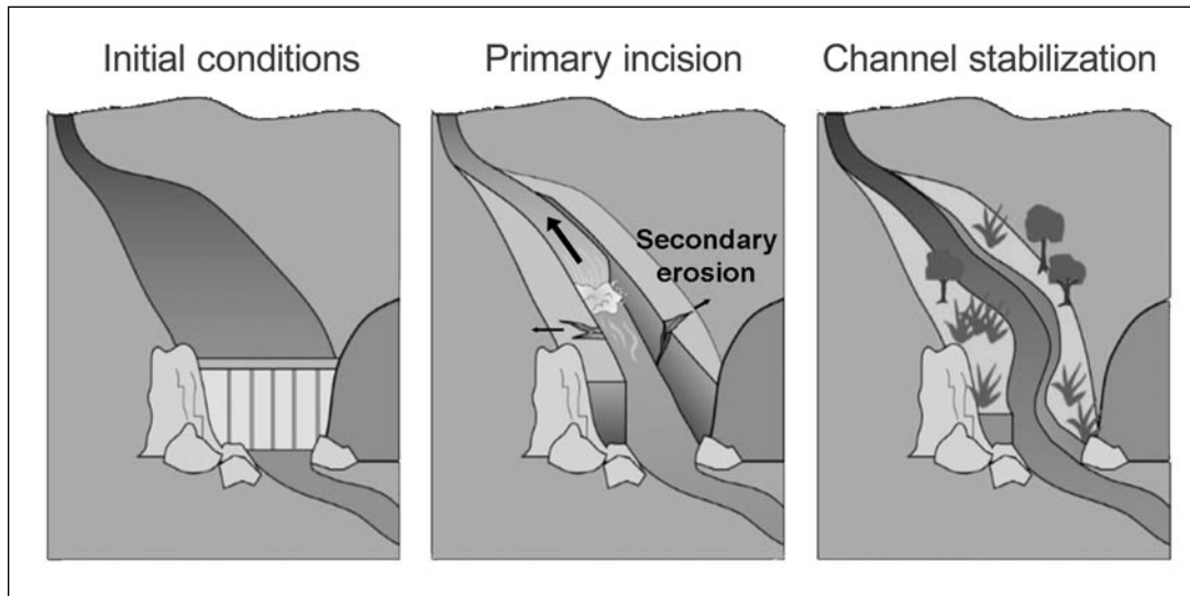
River recovery after a dam removal follows a predictable sequence of events. (Graphic by Shannon Hayes)
