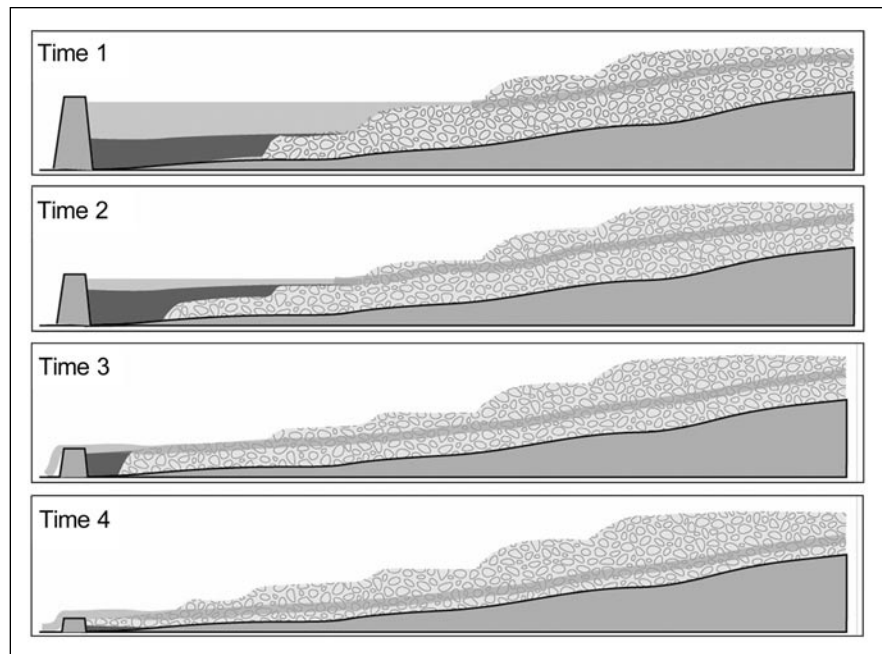
Large dams are removed incrementally from the top. As the reservoir behind the dam shrinks, the sediment marches forward toward the dam. (Graphic by K. Ronnenberg)
