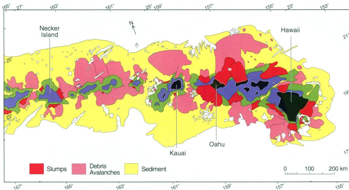
Shifting territory. Geologic interpretive map generated from GLORIA backscatter imagery of the Hawaiian Ridge showing the position of giant landslides.
