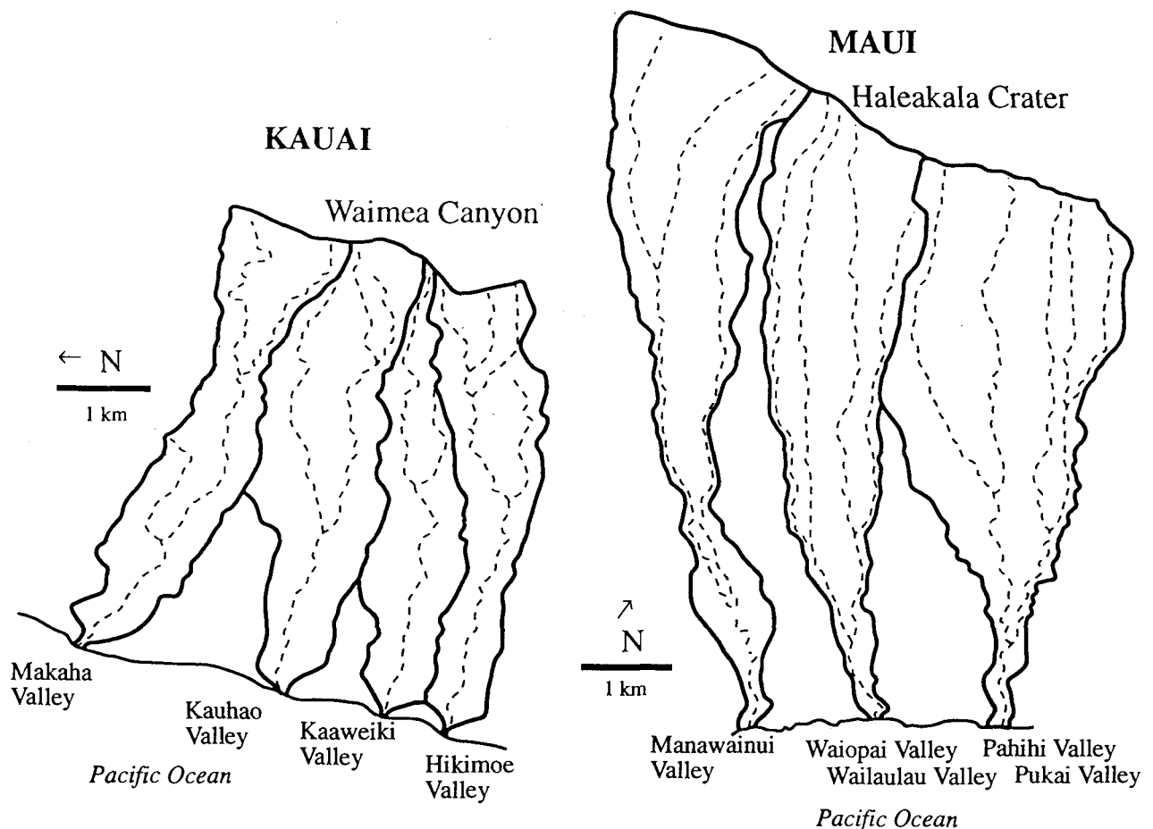
Figure 5. Outlines of drainage basins on Kauai and East Maui. Note that both drawings are at the same scale.
