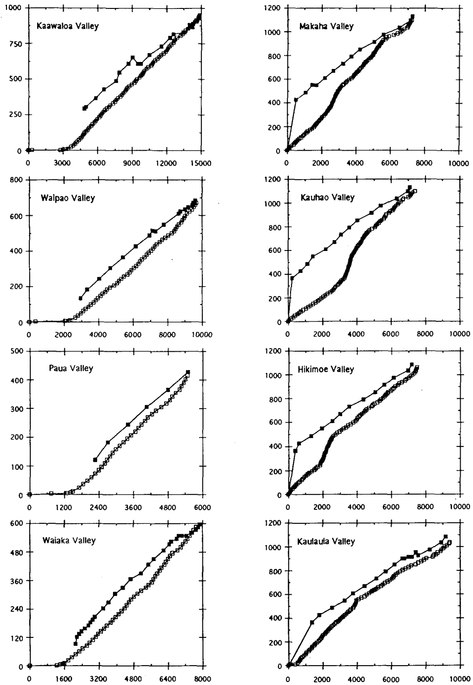
Figure 6. Representative profiles from Kauai with elevation and distance plotted in meters on the y- and x-axis, respectively. The straight to weakly convex Mana Plain profiles are shown on the left; the flat channel segments beginning at the sea correspond to the Mana Plain. Napali Coast channel profiles are shown on the right. Note the sharp knickpoints and longer convex reaches that punctuate the profiles. Open squares represent the channel profiles and solid squares represent the paleosurfaces above the channels. Note that the amount of vertical exaggeration differs from profile to profile.
