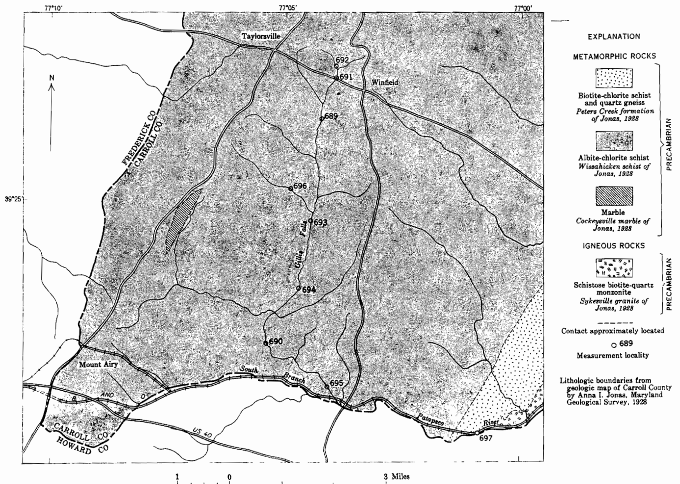
FIGURE 13.—Map of a part of Carroll County, Md., showing the location of measurements in Gillis Falls and the South Branch of the Patapsco River, and the distribution of major lithologic units.
