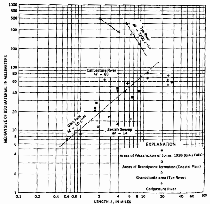
FIGURE 33.—Logarithmic graph showing the relation between median size of bed material and stream length for four streams in geologically different areas.
