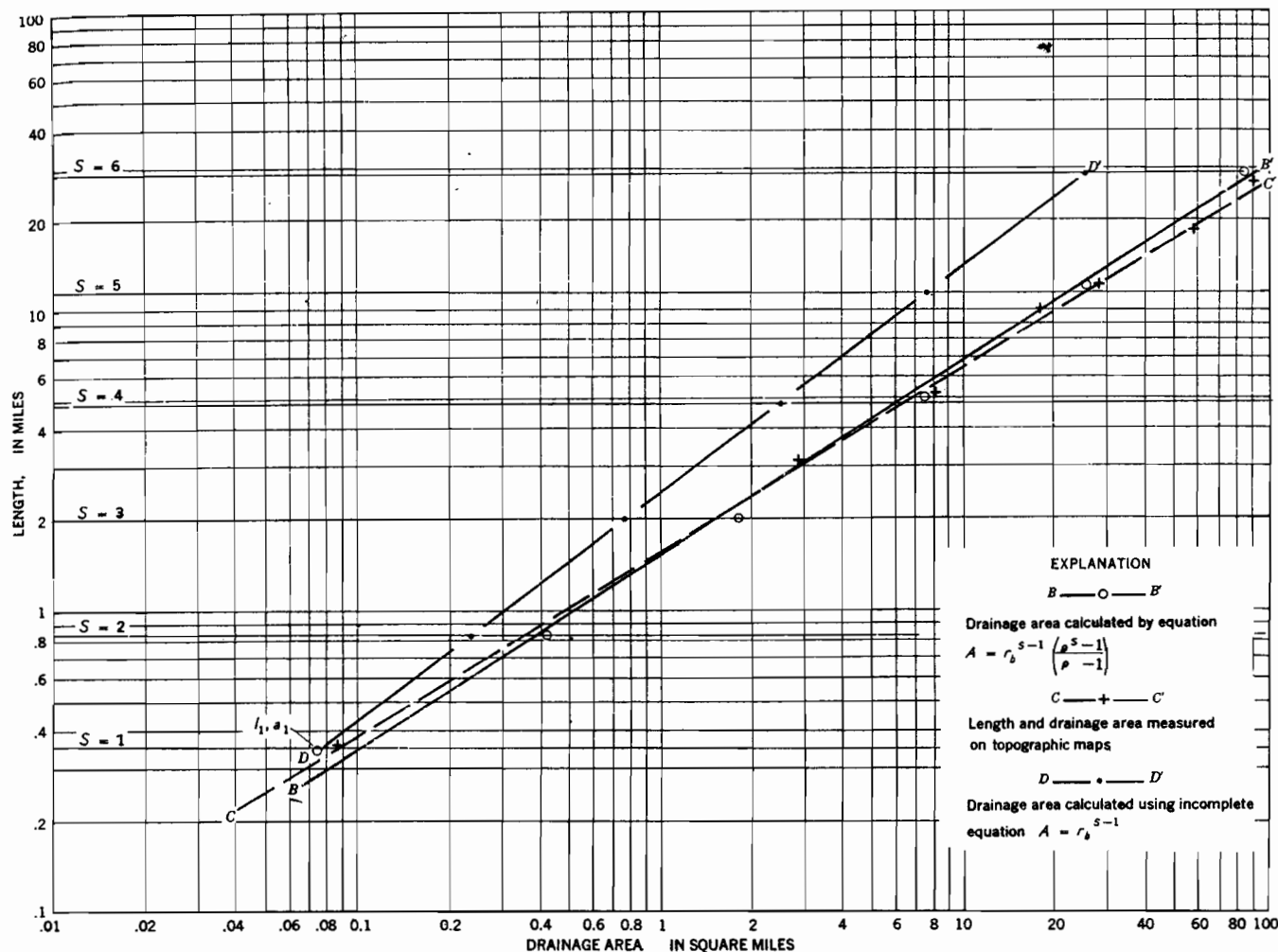
FIGURE 26.—Graph comparing calculated and measured values of stream length and drainage area in the watershed of Christians Creek, Va. B-B', line connecting calculated values based on a Horton analysis of stream lengths and number. C-C', line connecting measured values. See text for explanation of line D-D'.
