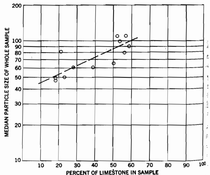
FIGURE 41.—Semi-logarithmic scatter diagram showing the relation between the median size of the entire sample of the bed material at the sampling localities and the percent of limestone in the sample.
