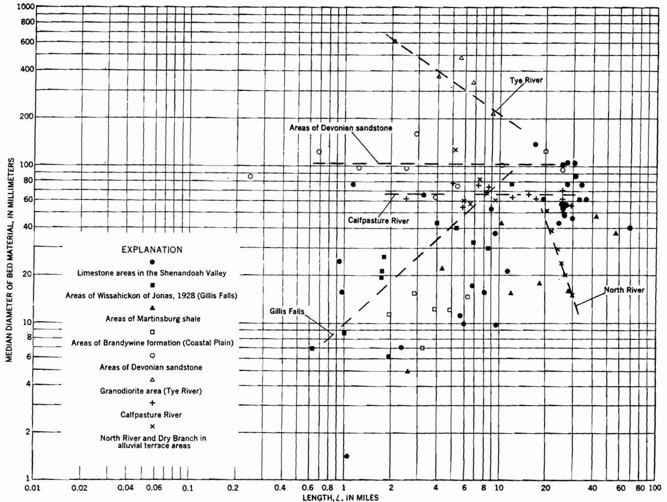
FIGURE 27.—Logarithmic scatter diagram showing the relation between length and median particle size of material on the stream bed at the measurement localities (table 8).
