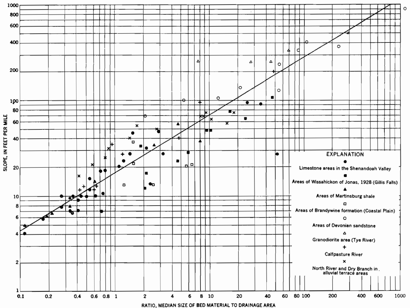
FIGURE 19.—Logarithmic graph showing the relation between channel slope and the ratio of median size of bed material to drainage area, at the measurement localities.
