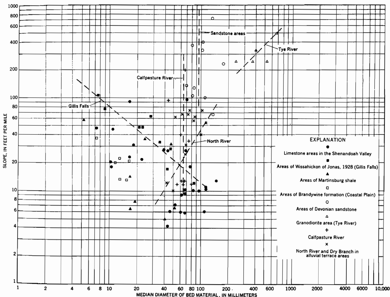
FIGURE 18.—Logarithmic scatter diagram showing the relation between channel slope and median size of bed material at the measurement localities (table 8).
